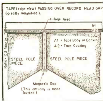
Fig. 3. Edge view of magnetic tape passing over recording-head gap, greatly enlarged.
