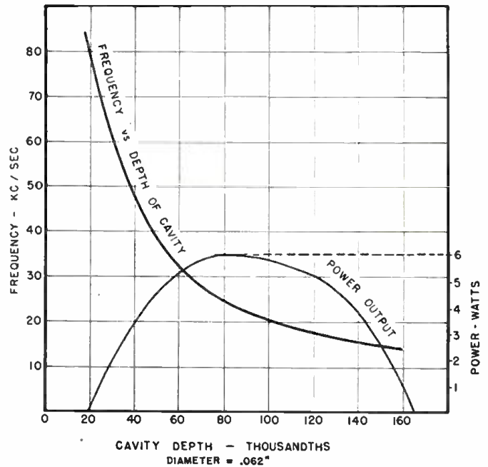
Fig. 5. Frequency and power output of cavity of varying depth. Cavity diameter = .062".
