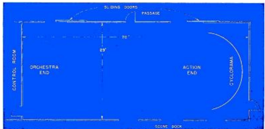
Fig. 2. Plan view, Studio A, London Television Station.
