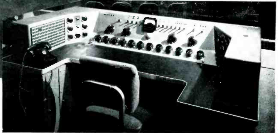
Fig. 3 (below). View of de luxe Studio A control console illustrating convenient location of all controls.
