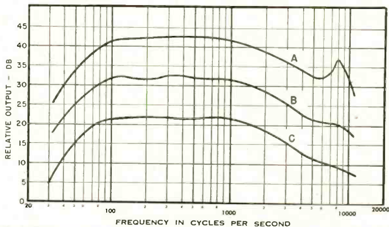
Fig. 3. Frequency response curves made from the same record with three different stylus radii.
