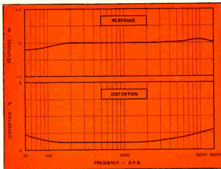
Fig. 4: Measured performance characteristics of portable amplifier.
