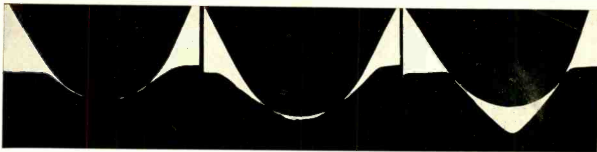
Fig. 2. Shadowgraph of stylus riding on bottom of groove, resulting in curve (A) of Fig. 3. Fig. 4. More nearly ideal groove fit, with curve (B) of Fig. 3. Fig. 5. Groove fit resulting from use of stylus too large for the groove being reproduced. Response curve (C).
