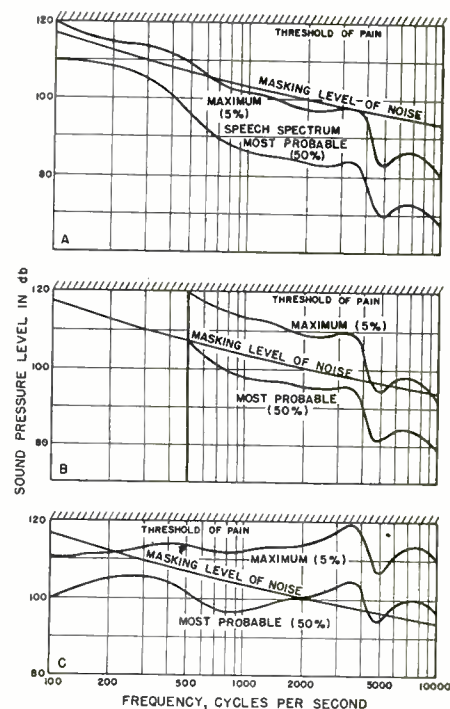
Fig. 10. The effect of transmission characteristics on the masking of declamatory speech by noise. (Courtesy Jensen Radio Mfg. Co.) A—Flat system frequency response. B—Flat system frequency response with cut-off at 500 cps. C—System frequency response rising 6 db per octave.
