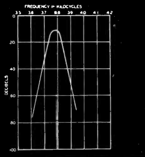
NARROW BAND SHARP CUTOFF FILTER
