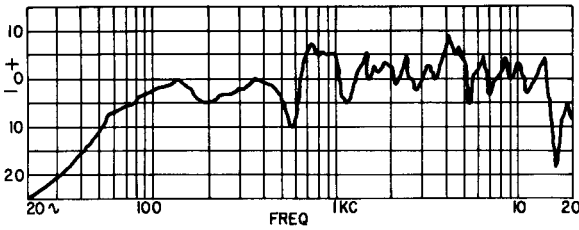
Fig. 113. Speaker response curves are quite different from those of amplifiers. The hill-and-valley nature of a speaker's response is shown in this typical curve.
