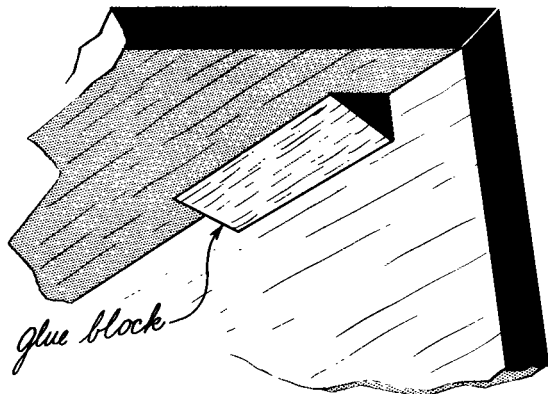
Fig. 117. Speaker enclosures have been known to come apart from vibration and air pressure caused by a speaker working at high levels. Brace the joints with glue blocks.
