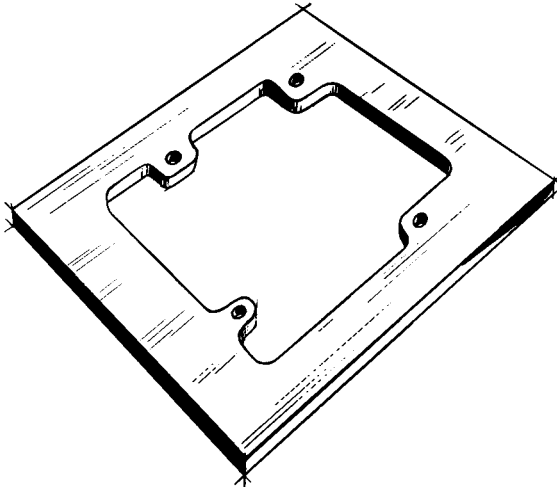
Fig. 102. For fixed installation of a record changer, a mounting board is used. It can be obtained pre-cut for various makes and models of changers or can be made with templates supplied by the manufacturer.
