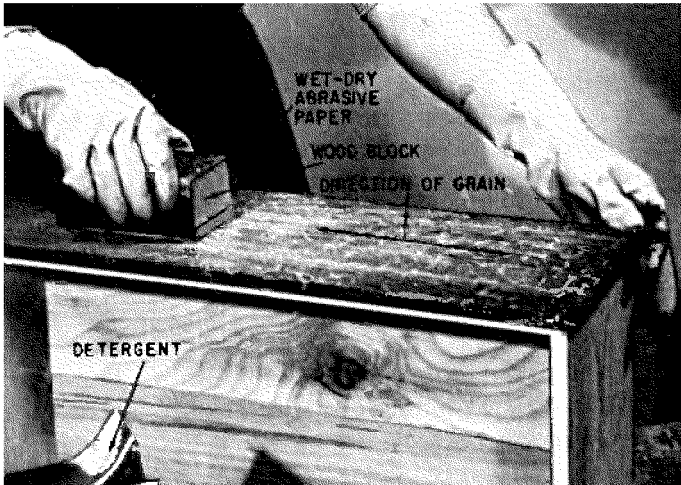
Fig. 708. Rubbing is an essential feature of furniture finishing for matte or high-gloss finishes. (Courtesy Grand Rapids Varnish Corp.)
