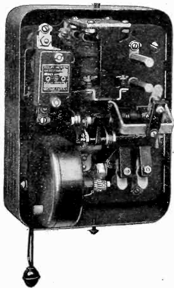
FIG. 24—DEFINITE-TIME AUTOMATIC STARTER FOR D-C. MOTORS
