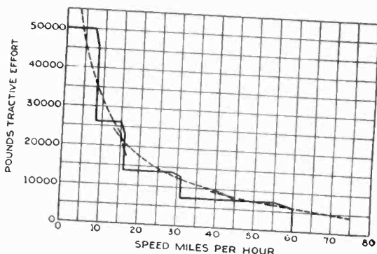
FIG. 1—SPEED-TRACTIVE EFFORT OF DIESEL LOCOMOTIVE
