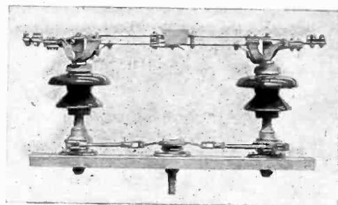
HORIZONTAL BREAK SWITCH
