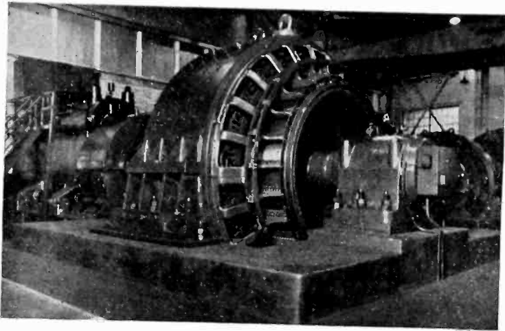
FIG. 8—A 7000-HP. D-C. REVERSING MILL INSTALLED AT THE YOUNGSTOWN SHEET AND TUBE COMPANY
