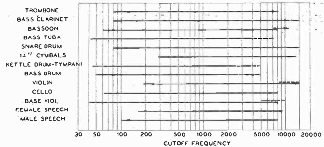
FIG. 2—SUMMARY OF IMPORTANT RANGES REQUIRED FOR DIFFERENT INSTRUMENTS
