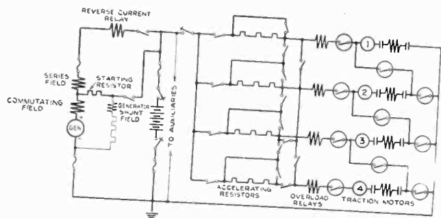
FIG. 16—CONNECTIONS FOR COMBINATION GENERATOR-BATTERY POWER PLANT
