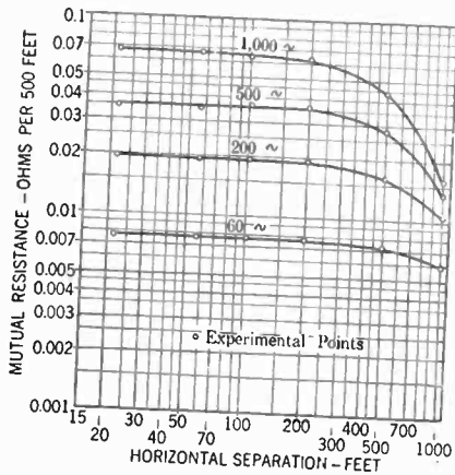
FIG. 2—CROSS KEYS TESTS—MUTUAL RESISTANCE
