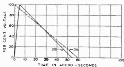
FIG. 2—PROPOSED STANDARD IMPULSE TEST WAVE
