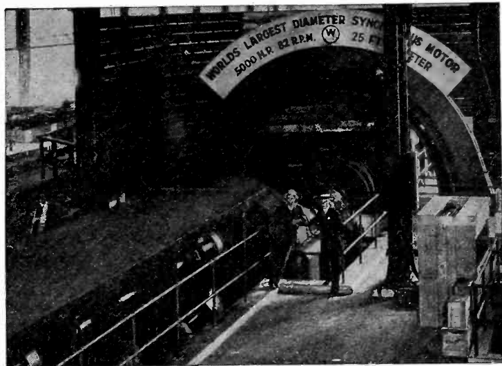
FIG. 7—A 5000-HP. SYNCHRONOUS MOTOR OF 25-FT. DIAMETER
