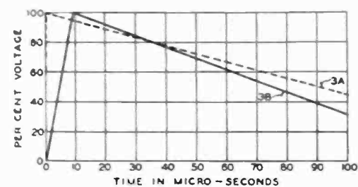
FIG. 3—PROPOSED STANDARD IMPULSE TEST WAVE
