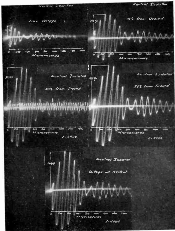
FIG. 9—OSCILLOGRAMS OF VOLTAGES IN A SHELL TYPE TRANSFORMER PRODUCED BY DAMPED OSCILLATIONS SIMILAR TO WITCHING
