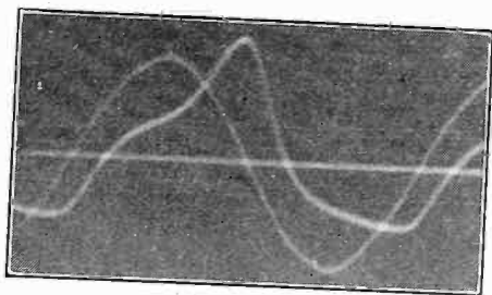
FIG. 6—PRIMARY VOLTAGE AND CURRENT IN A TRANSFORMER WHOSE CORE IS MAGNETIZED BY A DIRECT CURRENT IN THE SECONDARY
