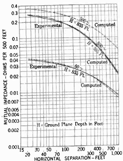
FIG. 7—CROSS KEYS TESTS GROUND PLANE THEORY
