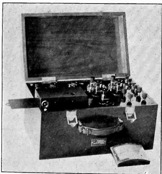
FIG. 3—OSCILLOGRAPH WITH CAMERA IN PLACE
