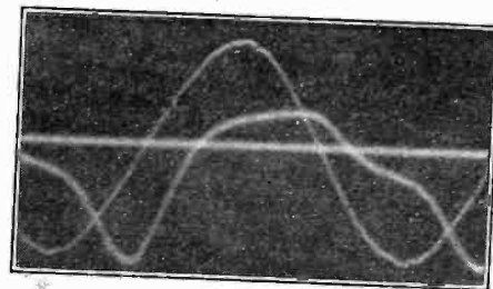
FIG. 8—PRIMARY VOLTAGE AND TRANSIENT MAGNETIZING CURRENT IN A TRANSFORMER IMMEDIATELY AFTER CLOSING THE PRIMARY CIRCUIT
