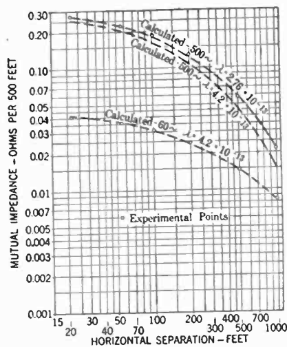
FIG. 13—CROSS KEYS TESTS—CARSON THEORY
