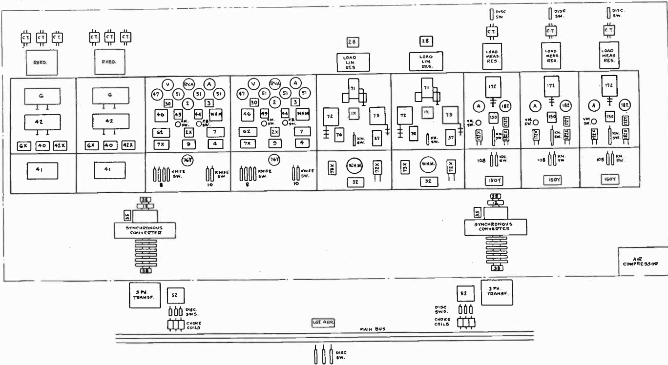
FIG. 1—SUBSTATION INSPECTION CHART
