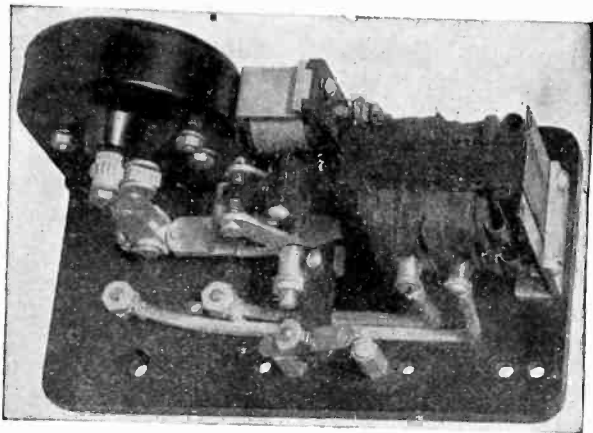
FIG. 23—FIELD RELAY FOR SYNCHRONOUS MOTOR WITH DEFINITE-TIME ELEMENT AND LOCKOUT COIL
