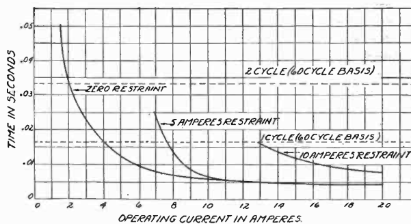
FIG. 5—TIME-CURRENT CURVES OF BALANCED CURRENT RELAY
