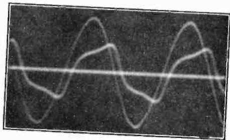
FIG. 5—OSCILLOGRAM OF PRIMARY VOLTAGE AND MAGNETIZING CURRENT IN A TRANSFORMER
