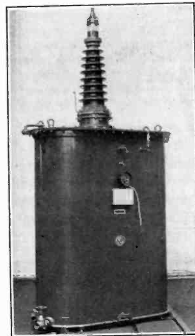
FIG. 19—IMPEDOR FOR BANK OF (3) 40,000-KV-A. 220-KV. TRANSFORMERS
