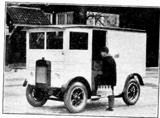
FIG. 26—GAS-ELECTRIC DELIVERY TRUCK IN DOOR-TO-DOOR SERVICE
