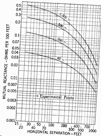
FIG. 3—CROSS KEYS TESTS—MUTUAL REACTANCE
