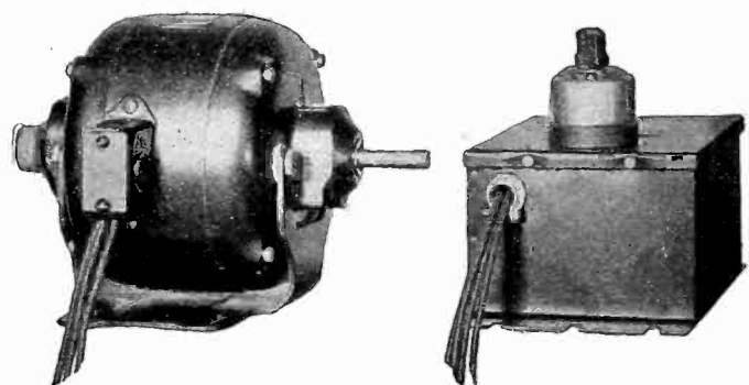
FIG. 27—1/4-HP. CAPACITOR MOTOR WITH THREE SPEEDS
