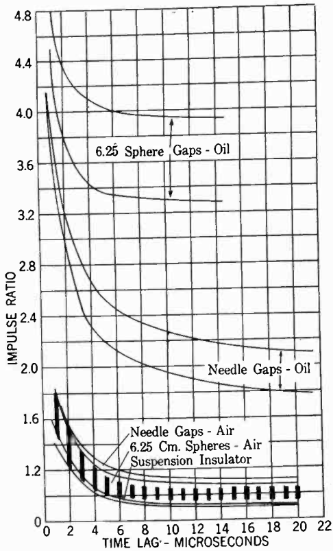
FIG. 4—IMPULSE RATIO CURVES FOR INSULATORS AND SPARK-GAPS
