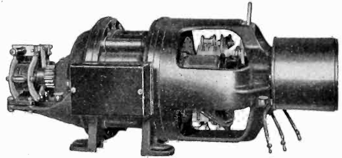
FIG. 25—3-HP. BRUSH-SHIFTING, ADJUSTABLE-SPEED, A-C. MOTOR
