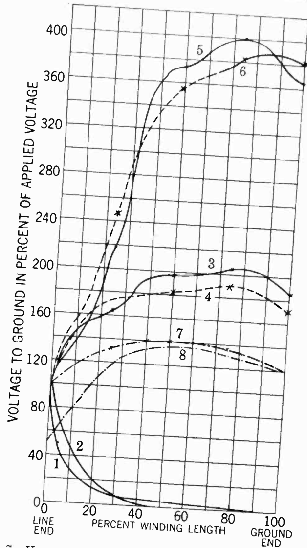
FIG. 7—VOLTAGE-TO-GROUND IN SHELL AND CORE TYPE TRANSFORMERS DUE TO LIGHTNING AND SWITCHING TRANSIENTS. (TEST)
