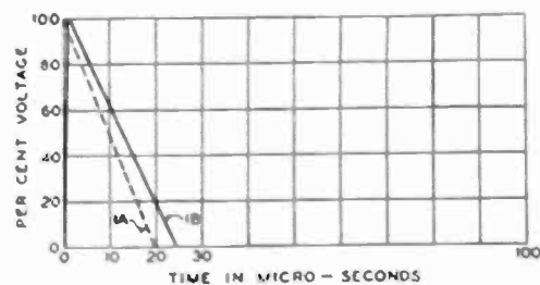
FIG. 1—PROPOSED STANDARD IMPULSE TEST WAVE
