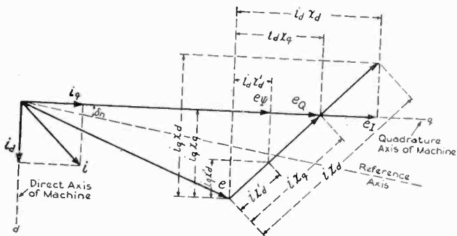
FIG. 8—VECTOR DIAGRAM OF STATOR VOLTAGES AND CURRENT OF A SYNCHRONOUS ALTERNATOR
