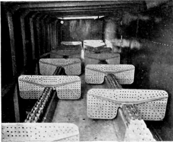
FIG. 3—PADDLE ARRANGEMENT OF CATERPILLAR TRACTOR TUGBOAT
