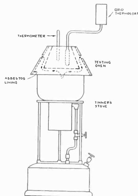
FIG. 2—FURNACE FOR TESTING THERMOSTATS
