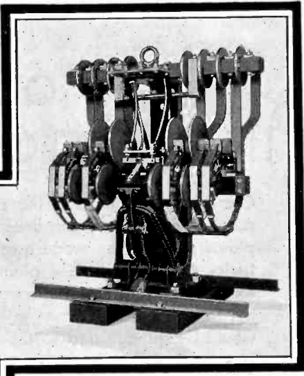
The single Type ZHS Magnetic Contactor, showing liberal electrical clearances, large bakelite barriers between phases and large contact areas.
