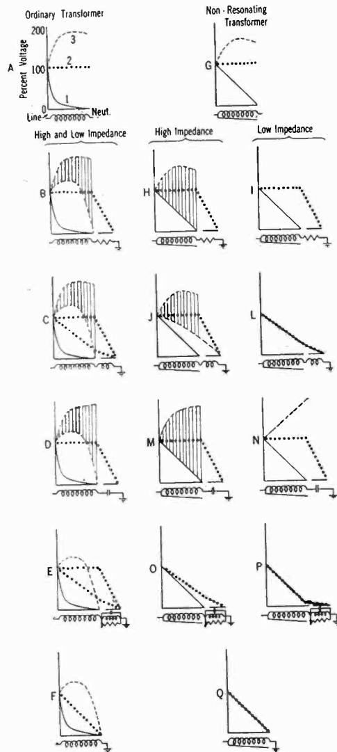
FIG. 3—SUMMARY OF EFFECT OF VARIATION OF NEUTRAL IMPEDANCE FROM ZERO TO INFINITY ON INTERNAL TRANSIENT VOLTAGES IN AN ORDINARY AND A NON-RESONATING TRANSFORMER PRODUCED BY TRAVELING WAVES MET IN SERVICE
