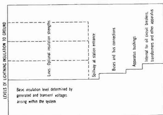
FIG. 1—DIAGRAMMATIC ILLUSTRATION OF RELATIVE LIGHTNING INSULATION STRENGTHS
