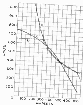
FIG. 3—ELECTRIC TRANSMISSION CHARACTERISTICS
