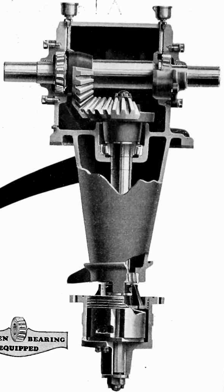
Roller Bearing Bevel Gear Assembly with Concentric Oil Dash Pot for Pacific Electric Floor Mounted Oil Circuit Breakers.
