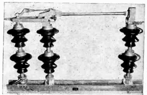
VERTICAL BREAK SWITCH
