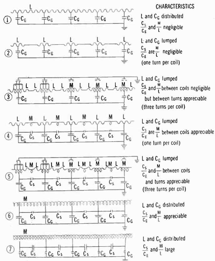
FIG. 1—SPECTRUM OF HIGH-FREQUENCY EQUIVALENT CIRCUIT
