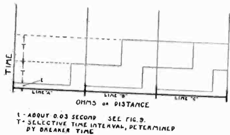
FIG. 6—STEPPED TIME CHARACTERISTICS FOR DISTANCE RELAY
