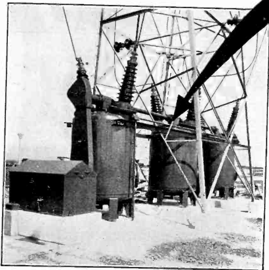
Pacific Electric 115 KV-600 Amp. Floor Mounted Type Oil Circuit Breaker.
