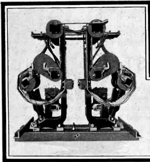
The double-contactor unit, mechanically interlocked, for reversing and plugging applications. Note the wide opening of contacts; this, combined with a high head and large volume of oil insures high arc-rupturing capacity.
