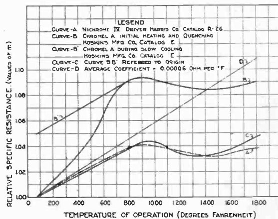
FIG. 1—RESISTANCE OF NICKEL-CHROMIUM AT ELEVATED TEMPERATURES
