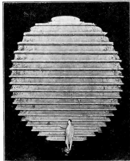
FIG. 2—ONE OF THE LOWER DEFLECTING VANE INSTALLATIONS
