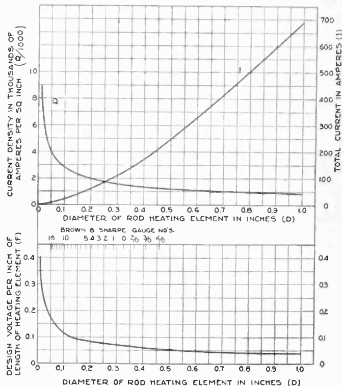
FIG. 5—DESIGN CURVES FOR NICKEL-CHROMIUM ROD HEATING ELEMENTS IN ELECTRIC FURNACES OPERATING AT 1850 DEG. FAHR. (BASED ON CURVE B, FIG. 4)
