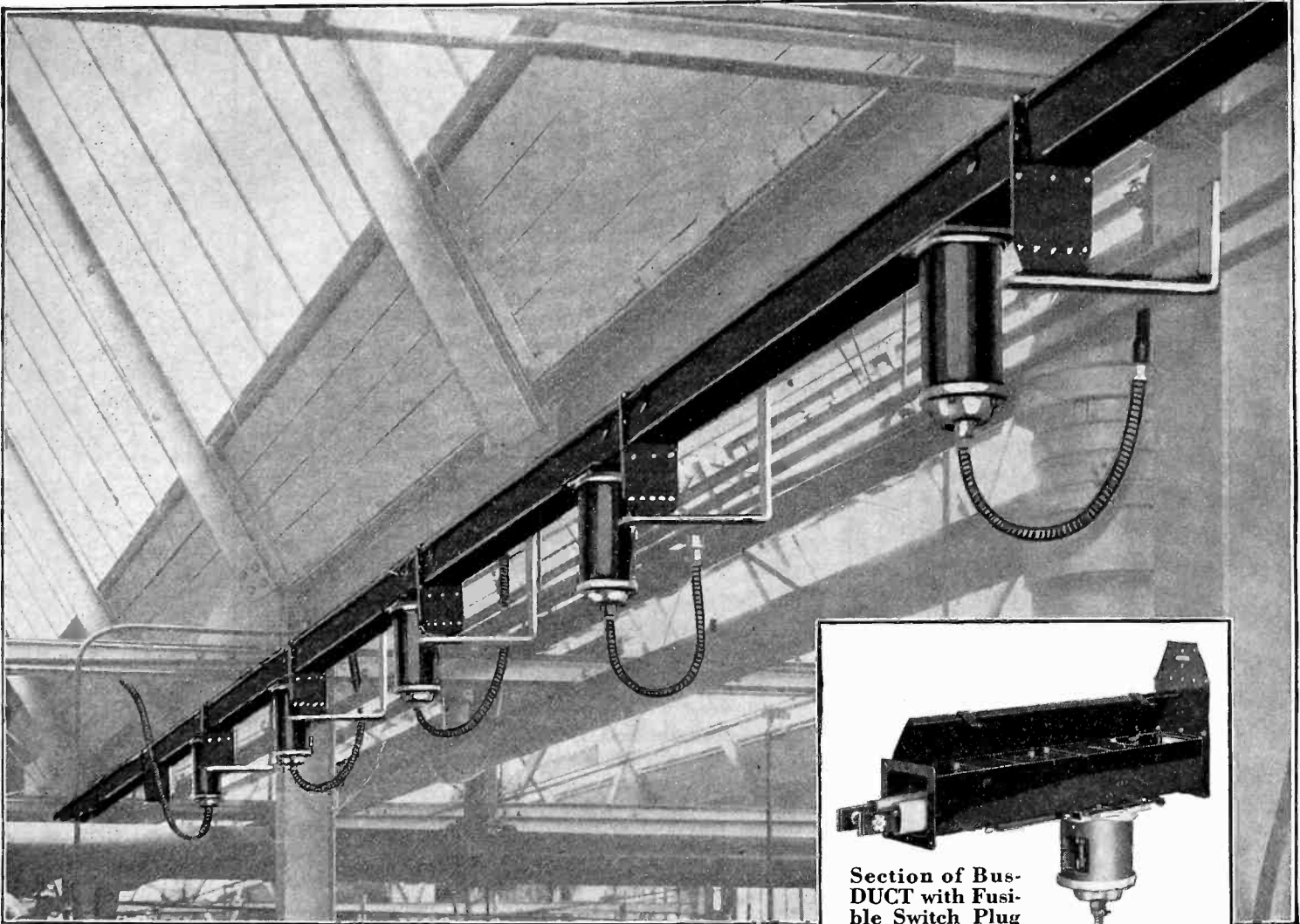
Bull Dog Bus-DUCT Installation in Graham Bros. Plant, Evansville, Ind.
