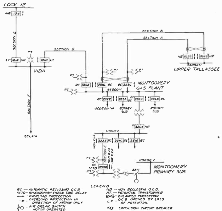
FIG. 4—MONTGOMERY AUTOMATIC SWITCHING SCHEME
