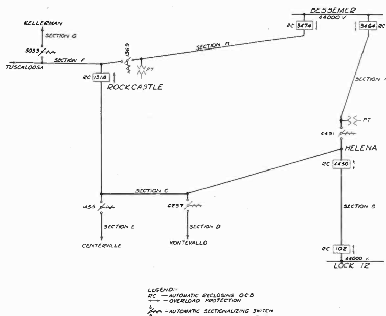
FIG. 1—BLOCTON LOOP AUTOMATIC SWITCHING SCHEME
