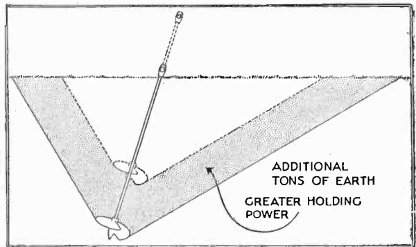
The shaded portion shows how greatly the cone of earth is increased in size by deeper installation, giving much greater holding power.
