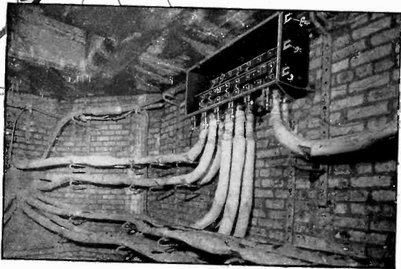
Below: Photo shows underground cable box assembly installed in Commonwealth Edison lines. Box fitted with Monel Metal bolts.
