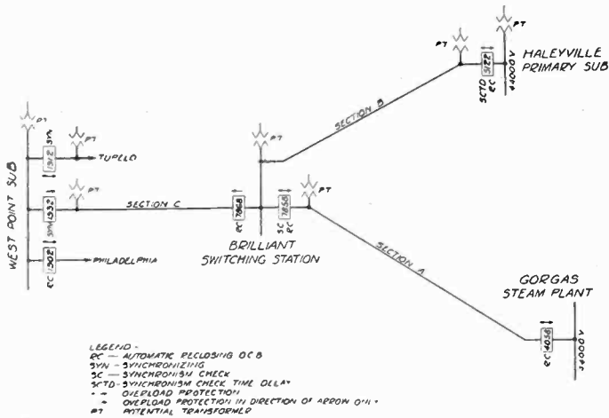
FIG. 2—ALABAMA-MISSISSIPPI AUTOMATIC SWITCHING SCHEME
