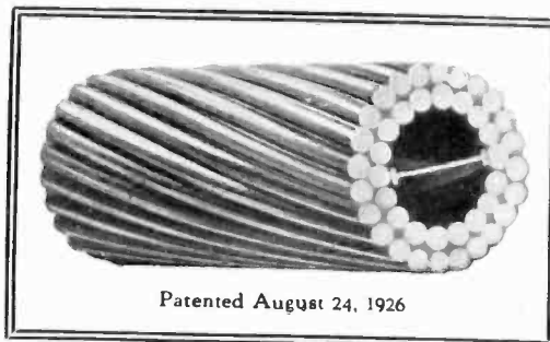
Side view of Anaconda Hollow Conductor showing the hollow construction.
