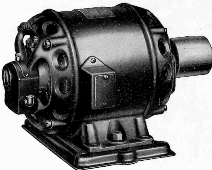
\frac{1}{4} Horse Power Century Type RS Repulsion Start Induction Single Phase Motor
