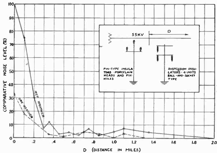
FIG. 1—ATTENUATION OF INTERFERENCE ALONG A TRANSMISSION LINE
