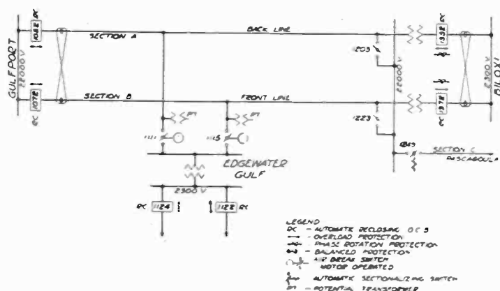
FIG. 6—GULFPORT-BILOXI AUTOMATIC SWITCHING SCHEME
