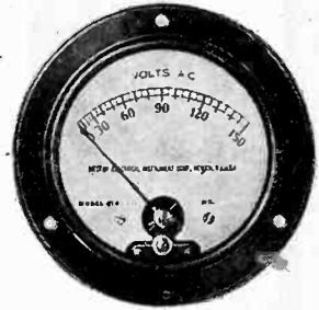
3 1/4" diameter A. C. panel type.
