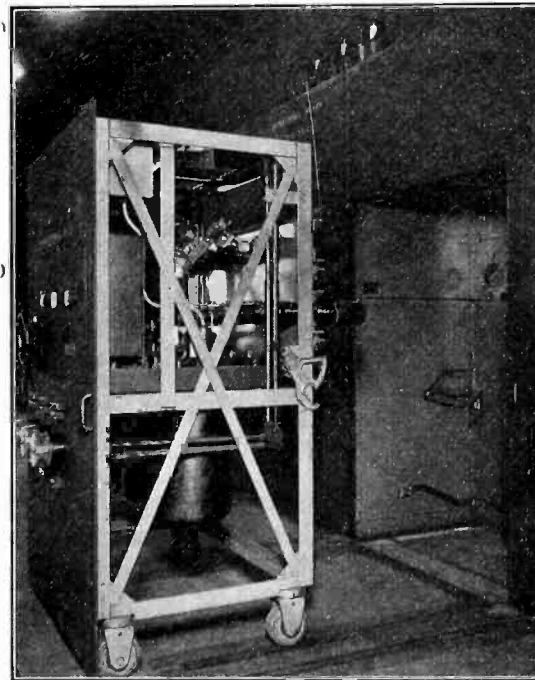
12,000-VOLT ENCLOSED SWITCH UNIT
