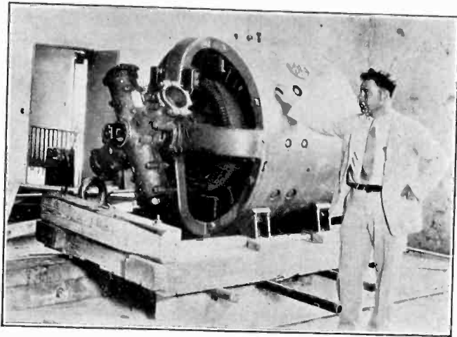
FIG. 3—PROPELLER MOTOR, 500 HP. CONTINUOUS RATING
