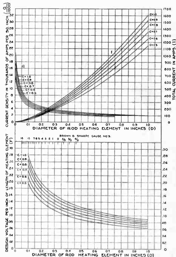
FIG. 3—THEORETICAL DESIGN CURVES FOR NICKEL-CHROMIUM ROD HEATING ELEMENTS IN ELECTRIC FURNACES OPERATING AT 1850 DEG. FAHR.
