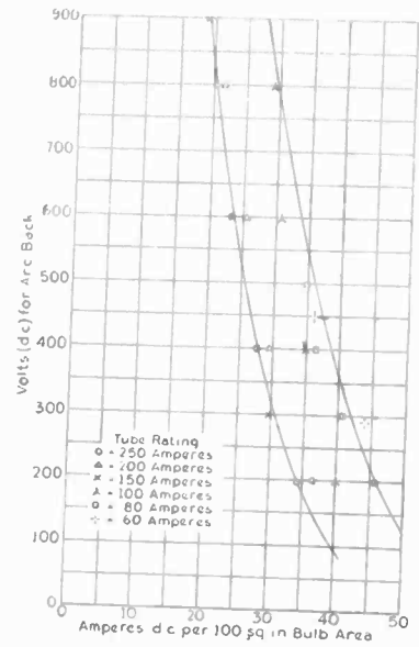
FIG. 13—COMPOSIT ARC-BACK CURVE FOR GLASS TUBES FAN-COOLED
