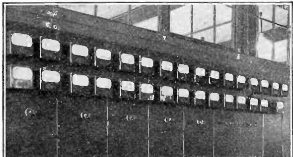
A Typical Insulation Showing Weston Rectangulars Mounted on Metal Panels
