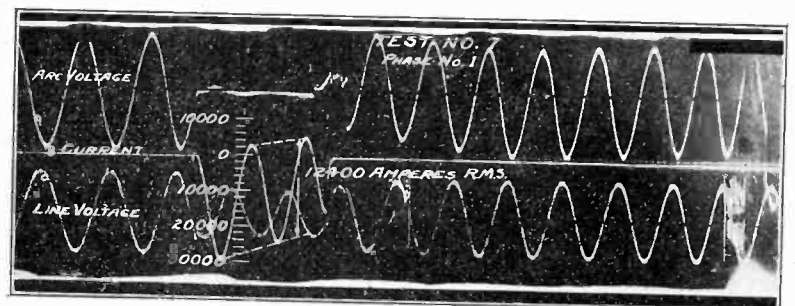
FIG. 15—OSCILLOGRAMS TAKEN ON TEST No. 7
