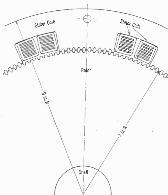
FIG. 2—SECTIONAL VIEW OF ALTERNATOR
