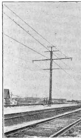
FIG. 15—TYPICAL 2-TRACK BRACKET CONSTRUCTION
