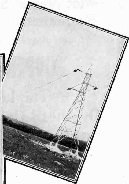
Anchor tower—Tennessee River crossing. Hales Bar-Richard City 44-kva. tie-line.
