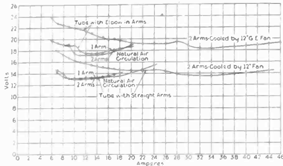
FIG. 1—ARC-DROP FOR 20-AMPERE GLASS TUBE
