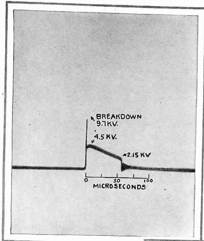
Volt-time characteristic of G-E pellet-type oxide film lightning arrester, recorded by the Dufour oscillograph
