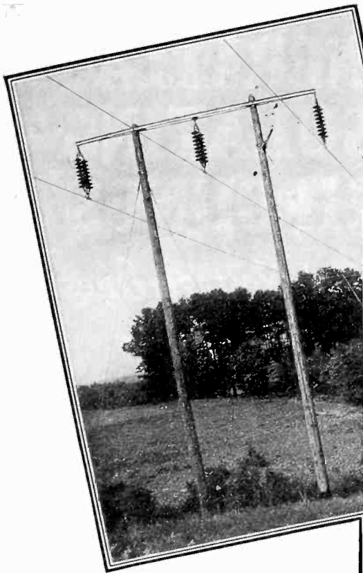
120,000-volt wood pole H-frame O-B Insulated line, Cleveland to Chattanooga. Yoked crossing for railroads.
