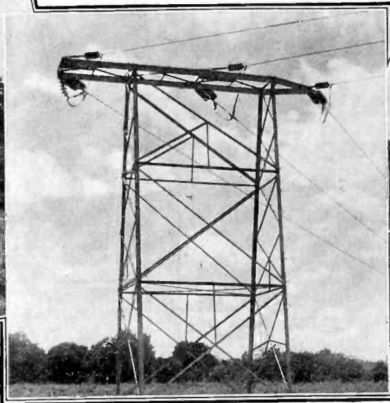
Anchor tower—Tennessee River crossing. Valdeau-Ridgedale 44-kva. tie-line.
