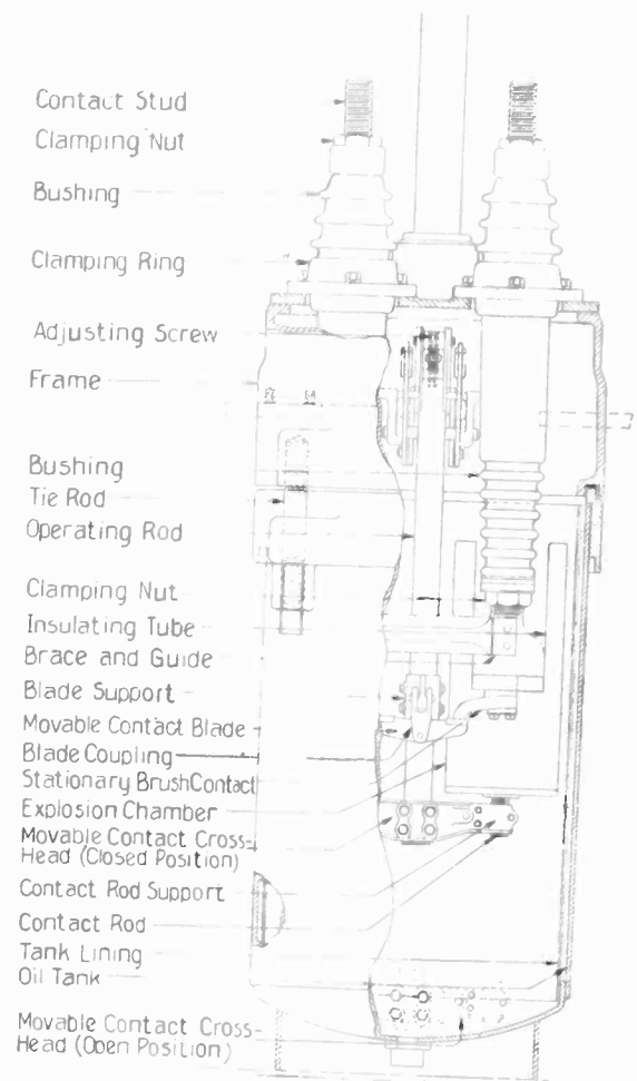
FIG. 3—SECTION OF ONE POLE OF THE BREAKER
