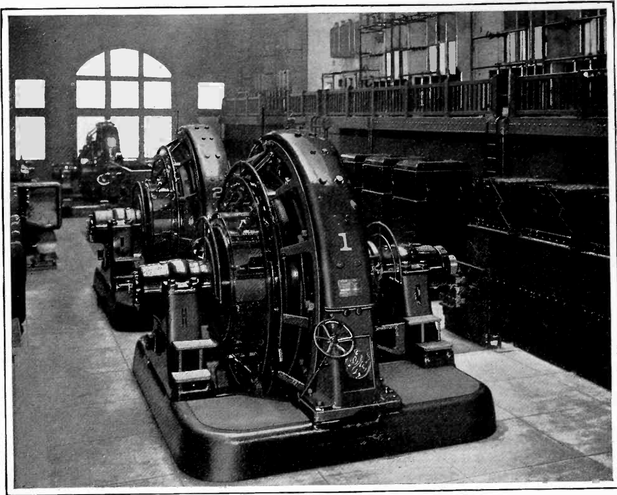
Irvington Substation, New York Central R. R.
