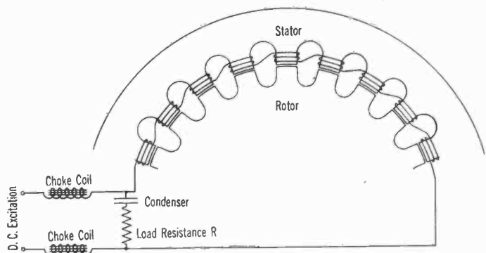
FIG. 1B—REACTION TYPE ALTERNATOR
