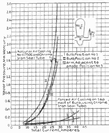
FIG. 8—VARIATION OF VAPOR PRESSURE WITH CURRENT IN GLASS RECTIFIER
