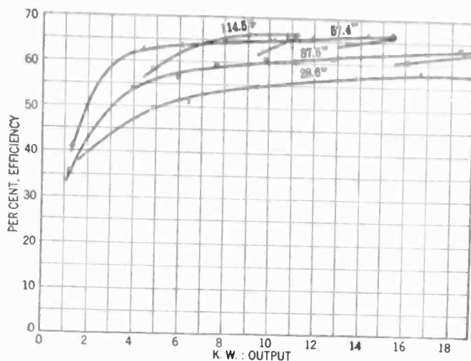
FIG. 5—VARIATION OF EFFICIENCY (EXCLUSIVE OF POWER REQUIRED FOR EXCITATION) WITH OUTPUT AND LOAD RESISTANCE
