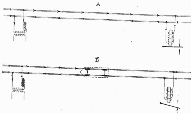
FIG. 2—ALTERNATING CURRENT TRACK CIRCUIT
