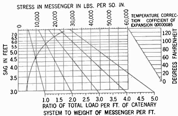
FIG. 7—MAIN MESSENGER DEFLECTION CURVE
