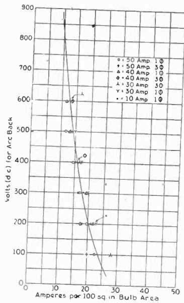
FIG. 12—COMPOSIT ARC-BACK FOR GLASS TUBES NATURAL AIR-COOLED
