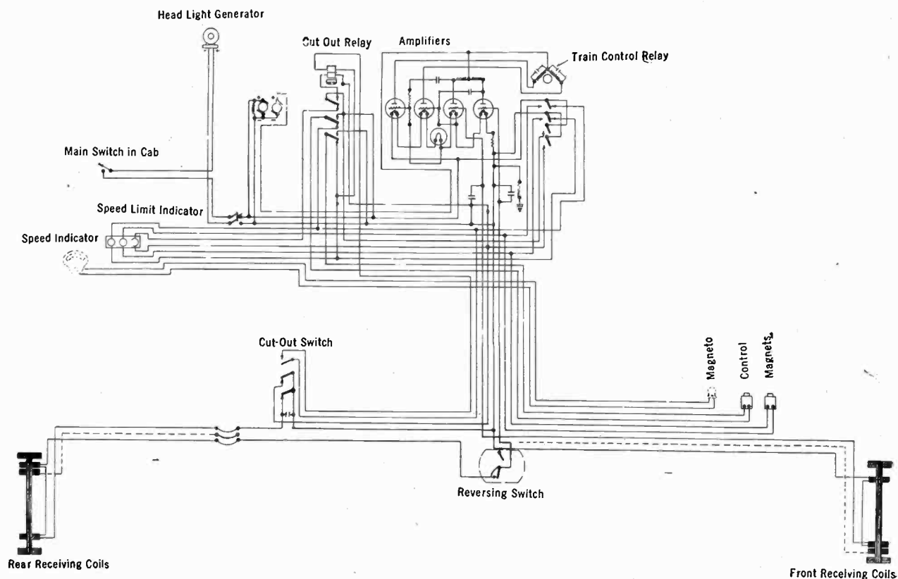
FIG. 5—CIRCUIT DIAGRAM AUTOMATIC TRAIN CONTROL
