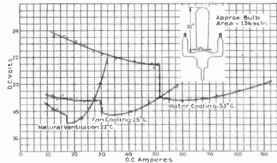
FIG. 4—EFFECT OF COOLING ON ARC-DROP OF 20-AMPERE GLASS TUBE
