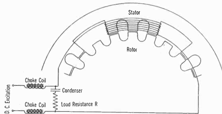
FIG. 1c—IMPROVED REACTION TYPE ALTERNATOR
