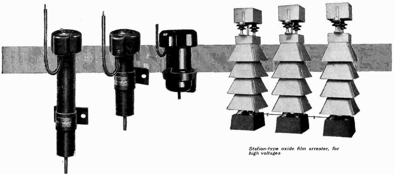
Pellet-type oxide film arresters of three different ratings. Built for voltages from 1000 to 50,000 volts
