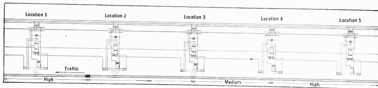
FIG. 6—TYPICAL TRAIN CONTROL ROADWAY CIRCUITS
