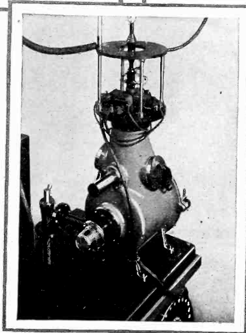
The Dufour Cathode-Ray Oscillograph, adapted by General Electric engineers to the photography of steep wave-front electrical transients
