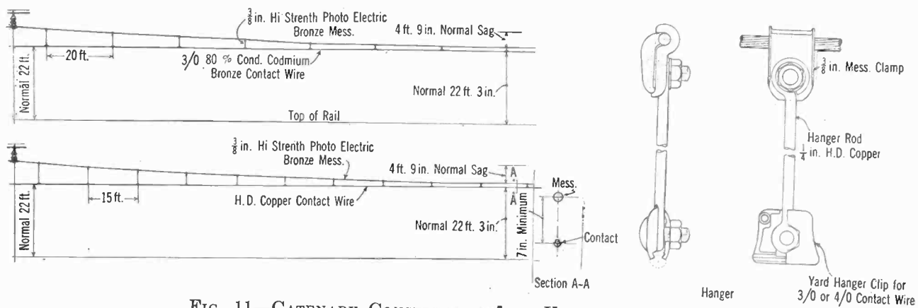
FIG. 11—CATENARY CONSTRUCTION FOR YARDS AND SIDINGS
