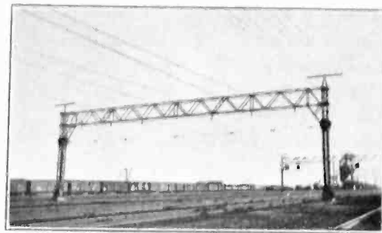
FIG. 17—TYPICAL 6-TRACK CONSTRUCTION
