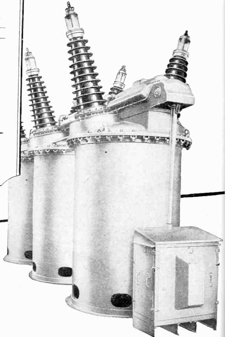
Type FHKO-39, 132,000-volt Oil Circuit Breaker
