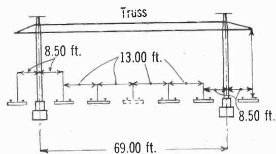
FIG. 3—TYPICAL ERECTION DIAGRAM
