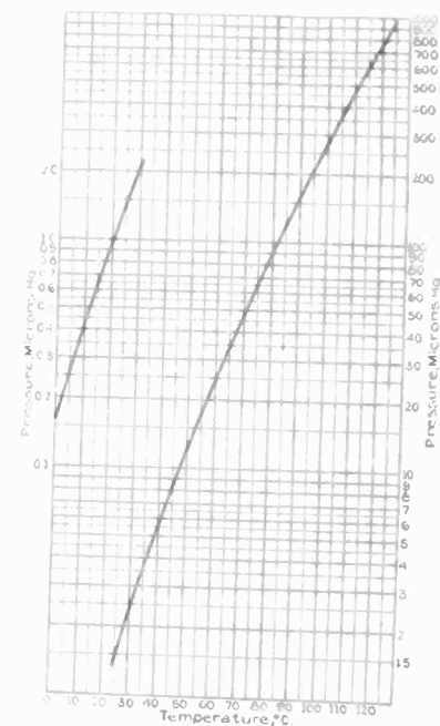
FIG. 7—TEMPERATURE AND PRESSURE OF SATURATED MERCURY VAPOR
