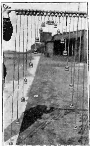
FIG. 14—COMPLETE SPAN OF HANGERS ASSEMBLED ON PIPE
