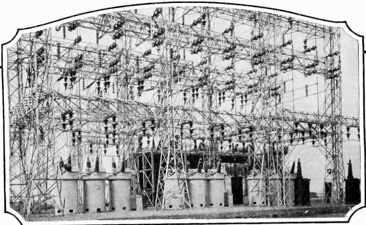
Type FHKO-39, 110,000-volt Oil Circuit Breakers in the Wilson Substation of the North American System, Merced, California
