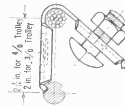
FIG. 10—TROLLEY WIRE CLIP
