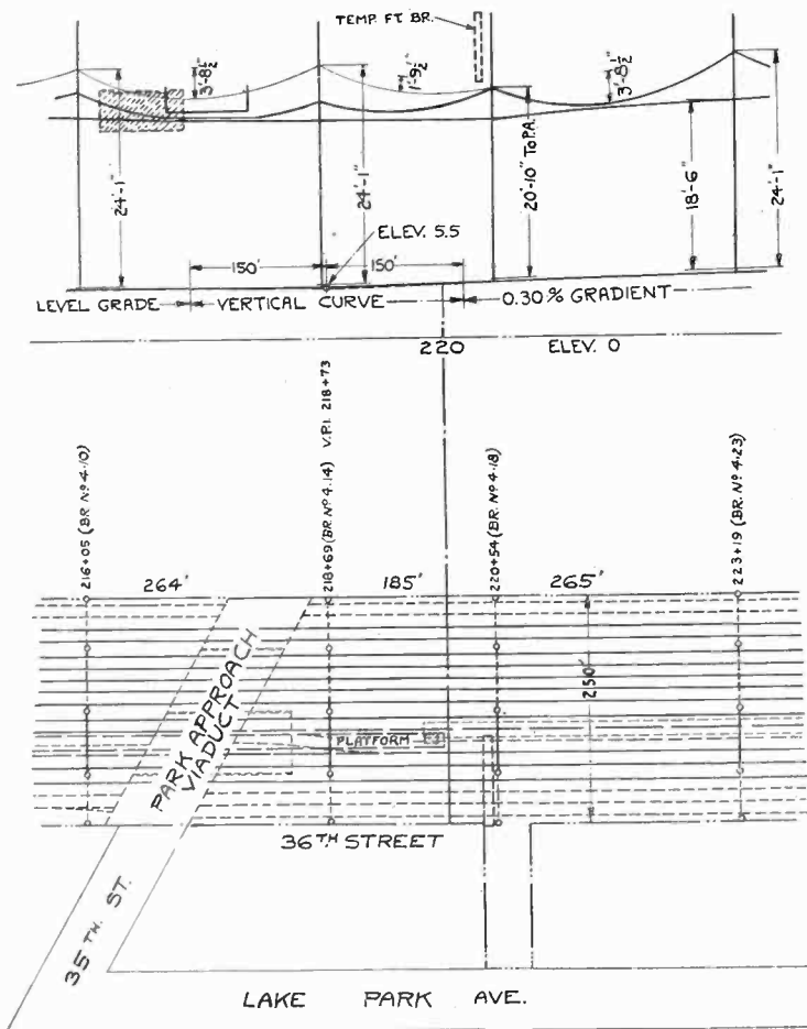
FIG. 1—TYPICAL TRACK PLAN
