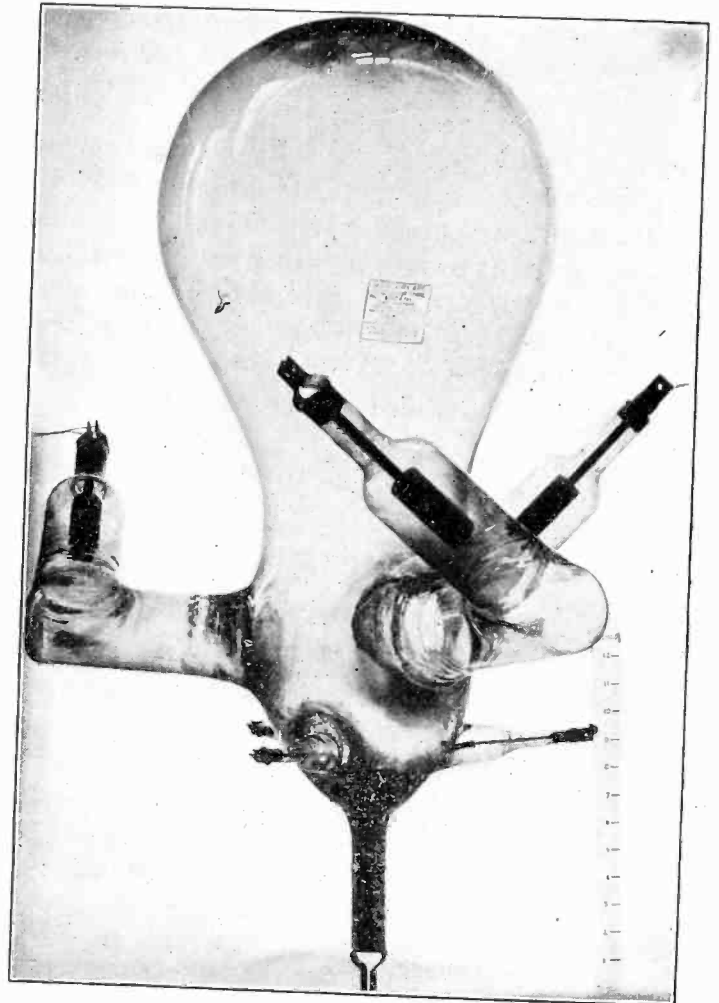
FIG. 14—250-AMPERE, THREE-PHASE 500- TO 600-VOLT MULTIPLE MERCURY ARC RECTIFIER TUBE
