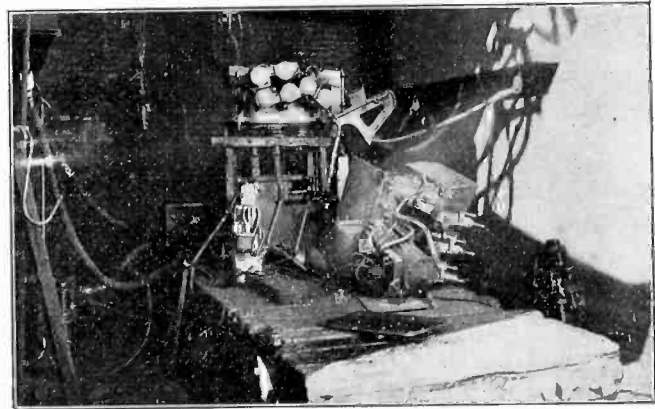
FIG. 17—REYROLLE SWITCHGEAR AFTER TEST NO. 7
