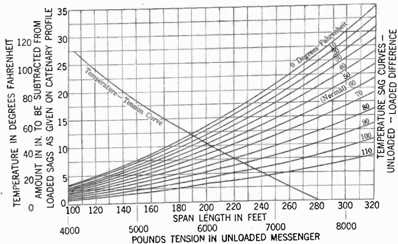
FIG. 12—TEMPERATURE—SAG CURVE
