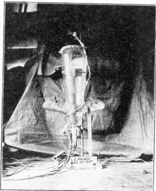
FIG. 6—50-AMPERE TUBE ARRANGED FOR VAPOR PRESSURE MEASUREMENTS
