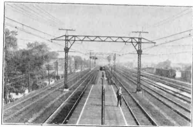
FIG. 16—TYPICAL 4-TRACK CONSTRUCTION
