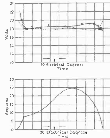
FIG. 3—INSTANTANEOUS ARC-DROP VARIATIONS
