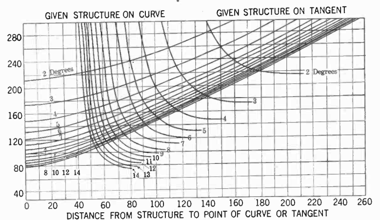
FIG. 2—SPACING CHART FOR STRUCTURES ON CURVES
