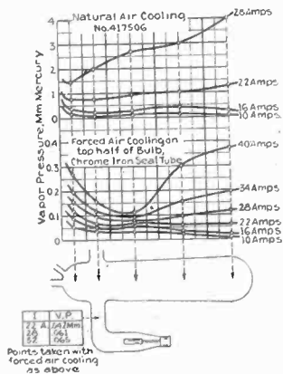
FIG. 9—VARIATION OF VAPOR PRESSURE WITH LOCATION IN GLASS RECTIFIER
