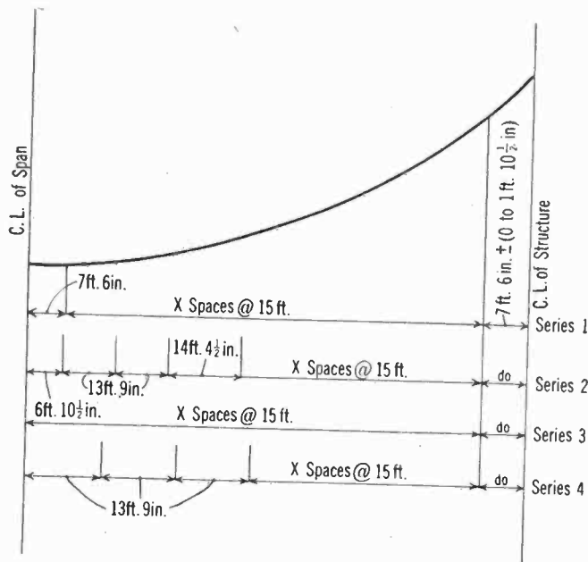
FIG. 9—CATENARY HANGER CHART
