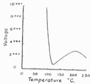
FIG. 19—BREAKDOWN OF MERCURY VAPOR
