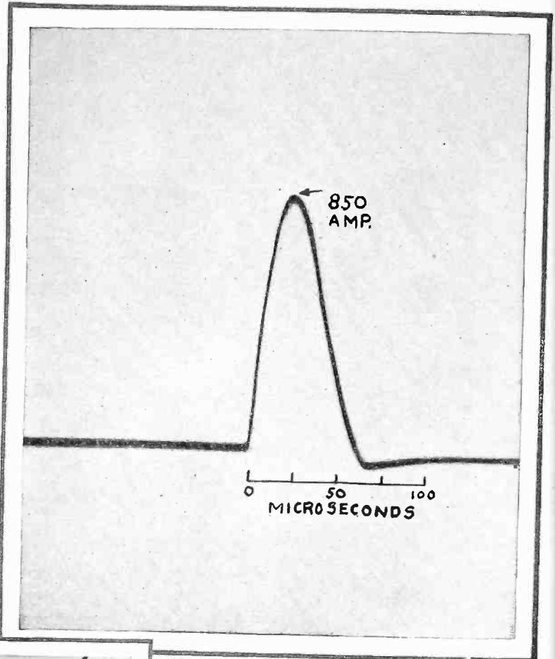
Ampere-time characteristic of G-E pellet-type oxide film lightning arrester showing the extremely short duration of the current flow
