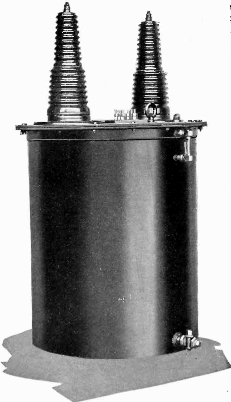
Typical American Transformer for Cottrell Precipitation Process
