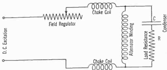
FIG. 3—CONNECTION DIAGRAM
