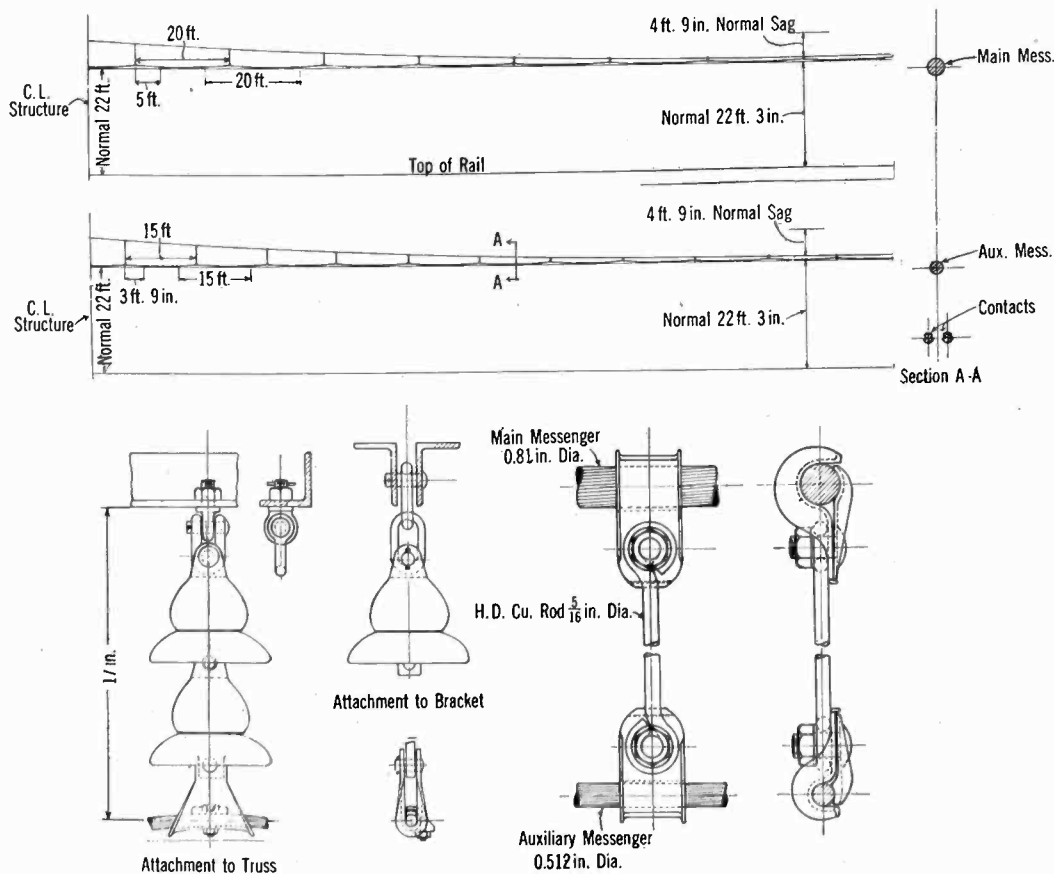
FIG. 8—MAIN LINE CATENARY SYSTEM
