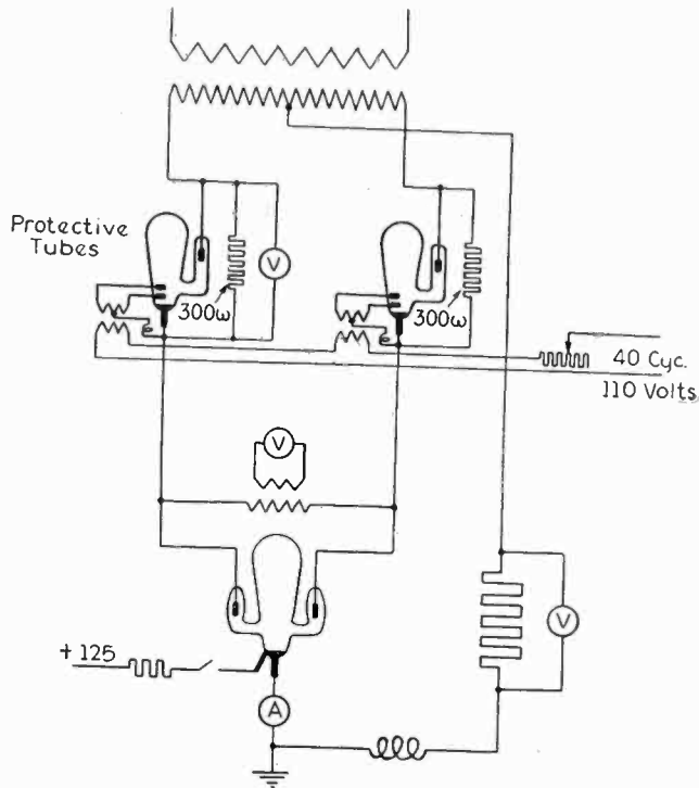
FIG. 11—ARRANGEMENT OF RECTIFIERS FOR ARC-BACK TESTS
