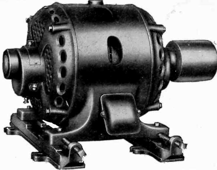
10 Horse Power Century Type AS Automatic-start Induction 3- and 2-phase Motor
