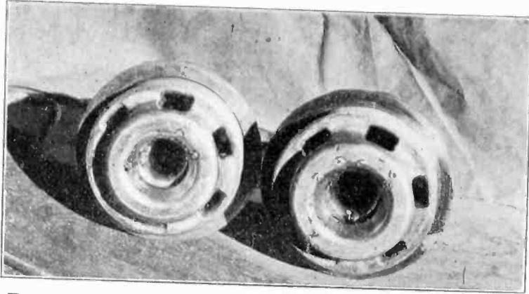
FIG. 27—CONTACTS FROM 136B BREAKER AFTER TEST NO. 31
