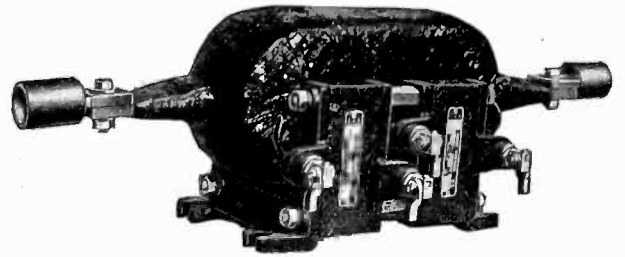
Type F-25 Sangamo Current Transformer with double secondary. This is only one of a great number of types. Ask for bulletin.
