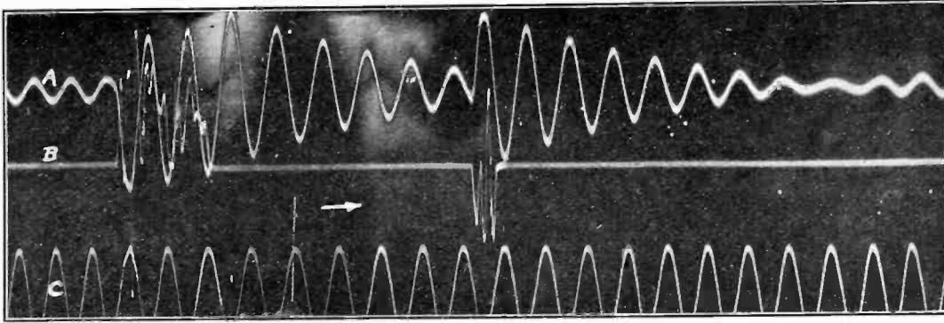
FIG. 28—C D 57304, SYSTEM LOADED, ALL LINES IN SERVICE. CONDUCTOR 1 GROUNDED AT LOCK 12 BY 1 AMPERE FUSE OVER PIN TYPE INSULATOR. NEUTRAL REACTOR SETTING 1088 OHMS
