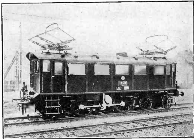
Prussian State Railways. Locomotive with direct-connected side rod drive with one motor through a vertical rod to the Jack cranks. Built by A. E. G., Berlin.
