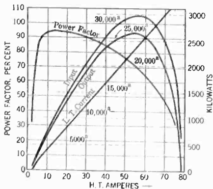
FIG. 3—CHARACTERISTICS OF ELECTRIC FURNACE FROM COMPLETE CIRCLE DIAGRAM
