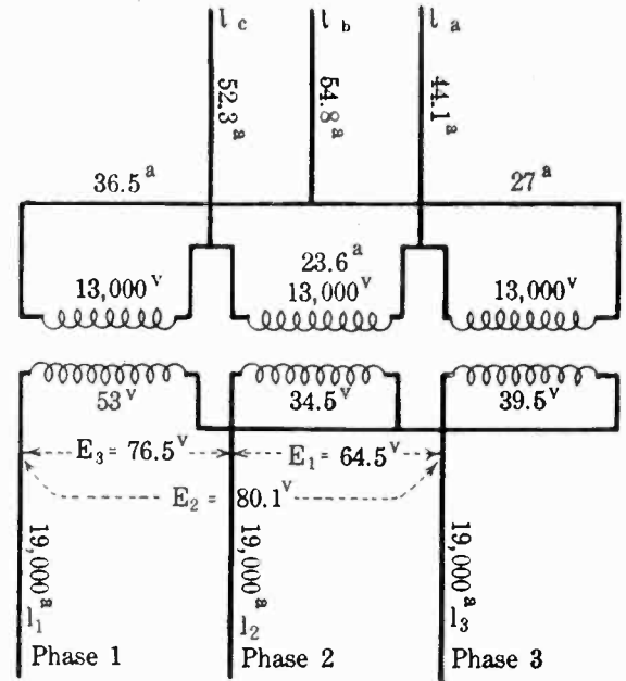
FIG. 8—DISTRIBUTION OF CURRENTS AND VOLTAGES
