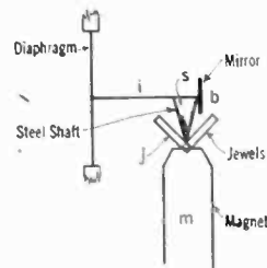
DETAILS OF VIBRATING SYSTEM
