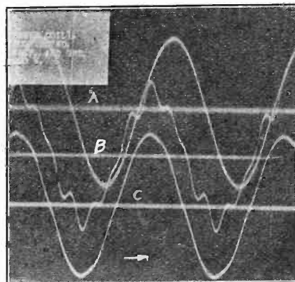
FIG. 19—C D 57282, TEST 5, LINE CHARGED, NO LOAD, REACTOR BETWEEN NEUTRAL AND GROUND
