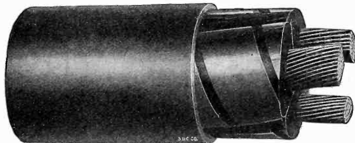
STANDARD Type H Cable for 25000 Volt Service (1/2 actual size) Note copper tapes around each core
