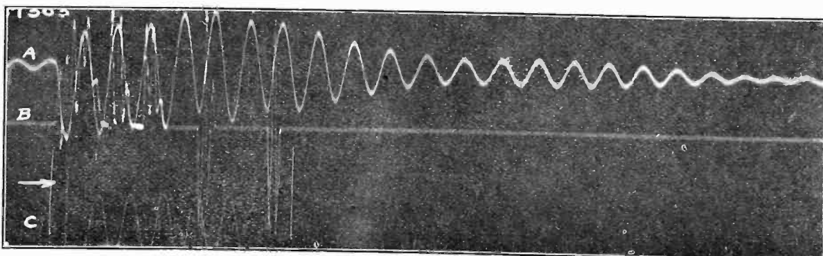
FIG. 27—C D 57303, SYSTEM LOADED, ALL LINES IN SERVICE. CONDUCTOR 1 GROUNDED AT LOCK 12 BY 1 AMPERE FUSE OVER PIN TYPE INSULATOR. NEUTRAL REACTOR SETTING 1207 OHMS.
