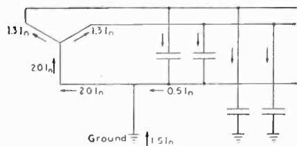
FIG. 8—CALCULATED FLOW OF CURRENT WITH ONE CONDUCTOR GROUNDED.
