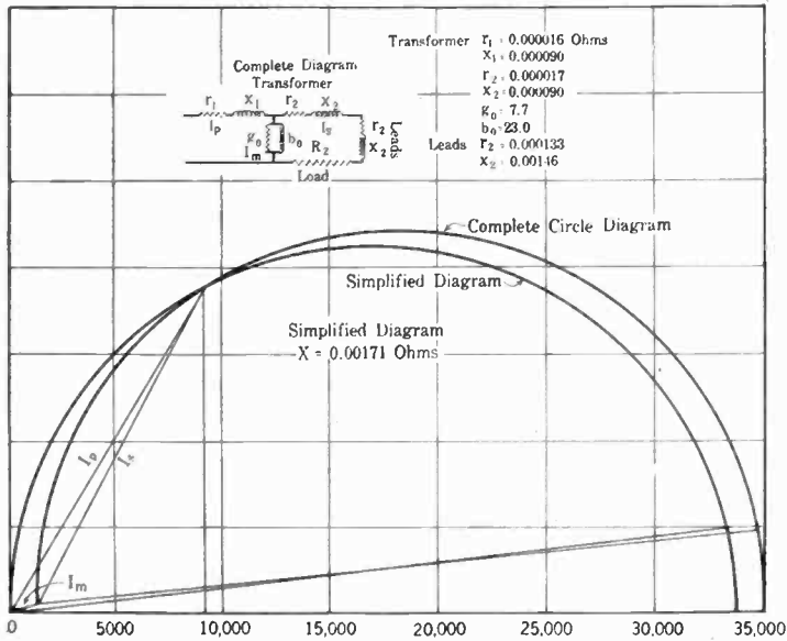
FIG. 2—COMPARISON BETWEEN SIMPLIFIED AND COMPLETE CIRCLE DIAGRAM
