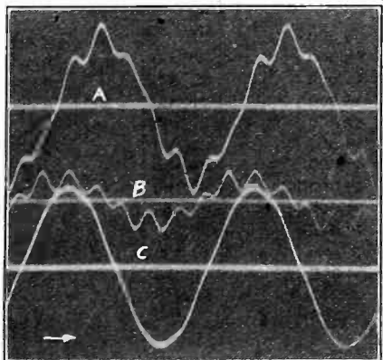
FIG. 17—C D 57279, TEST 4, LINE CHARGED, NO LOAD, NEUTRAL SOLIDLY GROUNDED
