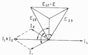
FIG. 4—VECTOR RELATION OF CURRENTS FLOWING IN CIRCUIT OF FIG. 3. ALL ANGLES MARKED BY ARROWS EQUAL 90 DEG.
