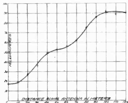
FIG. 58—OBSERVED CURRENT DISTRIBUTION IN 120 METER ANTENNA
