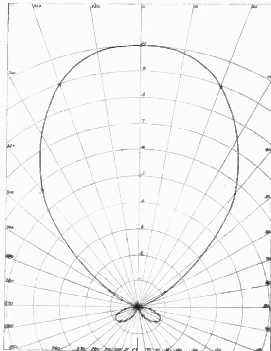
FIG. 44—DIRECTIVE CURVE OF WAVE ANTENNA. COMPENSATED BY REFLECTION FOR ZERO BACK END. \lambda = 12 KM., l = 12 KM., \alpha = 0.05 , u = 0.8 v
