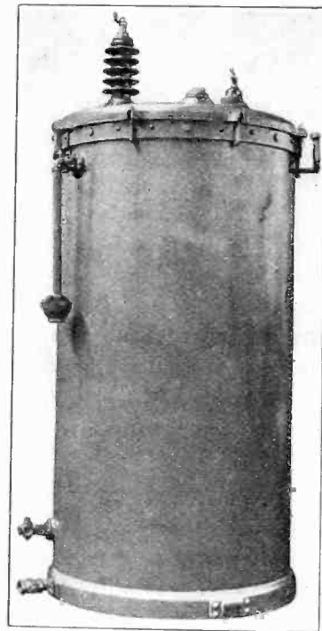
FIG. 11—EXTERNAL VIEW OF NEUTRAL GROUNDING REACTOR
