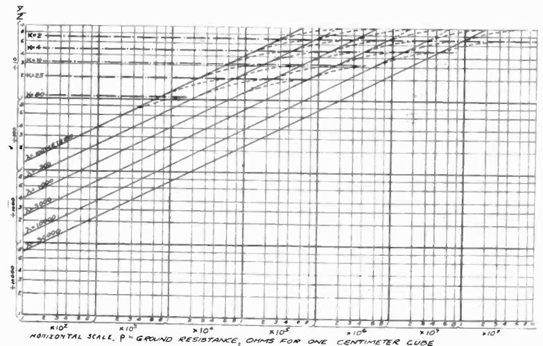
FIG. 55—WAVE FRONT TILT, X/Z BY ZENNECK'S FORMULA
