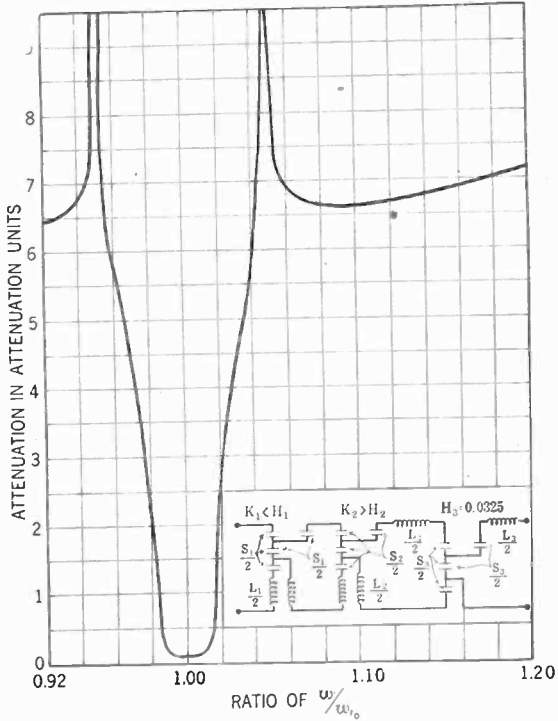
FIG. 21—ATTENUATION CURVE FOR COUPLED CIRCUIT WAVE FILTER
