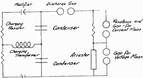
FIG. 7—CONNECTIONS FOR SURGE TESTS
