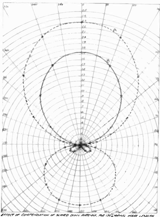
FIG. 52—A UNCOMPENSATED. B COMPENSATED. l = 3 \text{ KM.}, \lambda = 18, \alpha = .05, n = 0.333
