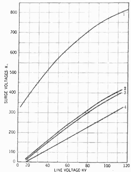
FIG. 2—VOLTAGE RELATIONS
