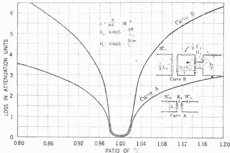
FIG. 19—ATTENUATION CURVES FOR BAND PASS WAVE FILTER
