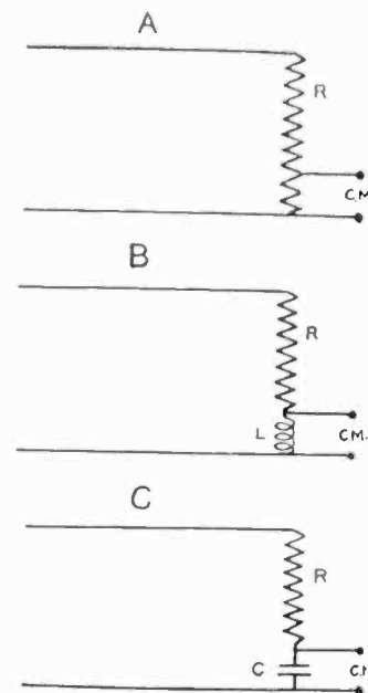
FIG. 3—CONNECTIONS FOR MEASURING PROPERTIES OF VOLTAGE WAVES
