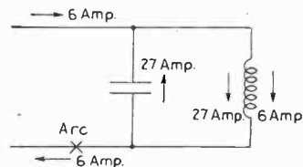
FIG. 38—EQUIVALENT DIAGRAM, SHOWING RESONANT CIRCUIT
