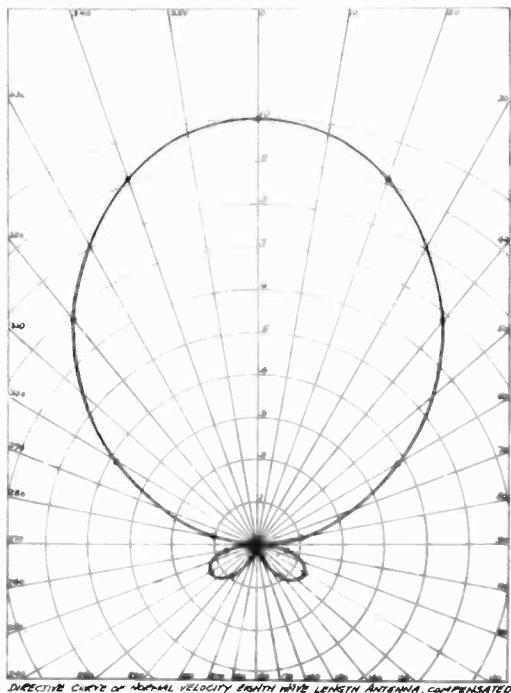
FIG. 51— l = 1.5, \lambda = 12, \alpha = 0.5, n = 0.8
