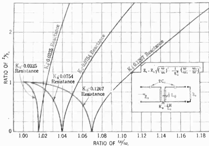
FIG. 7—CHARACTERISTIC IMPEDANCE FOR COUPLED CIRCUIT WAVE FILTER
