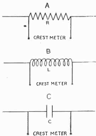
FIG. 2—CONNECTIONS FOR MEASURING PROPERTIES OF CURRENT WAVES
