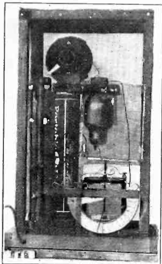
FIG. 9—SHIELDED CREST METER, WITH WINDOW TO INTERIOR OPEN
