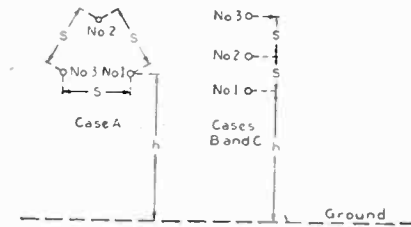
FIG. 7—ARRANGEMENT OF TYPICAL CIRCUITS FOR CALCULATING THE CAPACITANCE TO GROUND BY MEANS OF MAXWELL'S COEFFICIENTS
