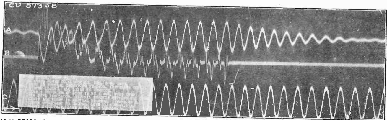
FIG. 32—C D 57308, SYSTEM LOADED, ALL LINES IN SERVICE. CONDUCTOR 1 GROUNDED AT LOCK 12 BY 1 AMPERE FUSE OVER PIN TYPE INSULATOR. NEUTRAL REACTOR SETTING 811 OHMS
