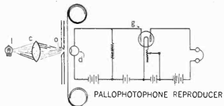
FIG. 8—DIAGRAM OF THE PALLOPHOTOPHONE REPRODUCER
