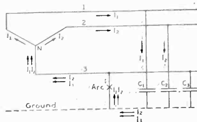
FIG. 1—THREE-PHASE SYSTEM WITH AN ARC FROM PHASE 3 TO GROUND. FIGURE SHOWS FLOW OF CURRENTS
