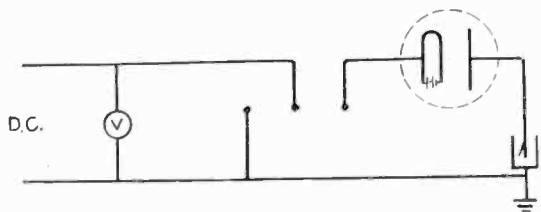
FIG. 6—CIRCUIT FOR CALIBRATION OF CREST METER
