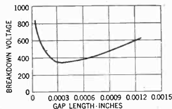
FIG. 1—BREAKDOWN VOLTAGE OF SMALL GAPS IN AIR
