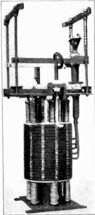
FIG. 12—INTERNAL VIEW OF NEUTRAL GROUNDING REACTOR
