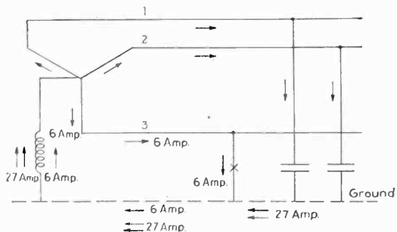
FIG. 37—THREE-PHASE CIRCUIT WITH NEUTRAL GROUNDING REACTOR OHMS OFF BALANCE. ASSUMED FLOW OF CURRENTS
