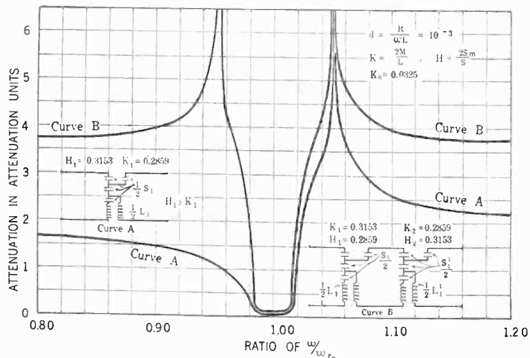
FIG. 20—ATTENUATION CURVES FOR COUPLED CIRCUIT WAVE FILTERS
