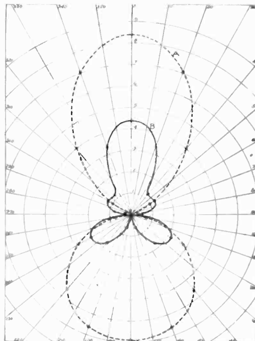
FIG. 53—A UNCOMPENSATED. B COMPENSATED. l = 3, \lambda = 8, \alpha = 0.5, n = 0.333
