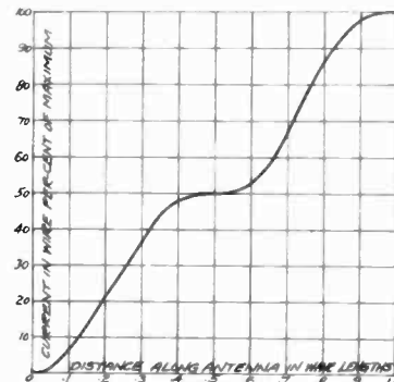
FIG. 59—CALCULATED CURRENT DISTRIBUTION IN WAVE ANTENNA
