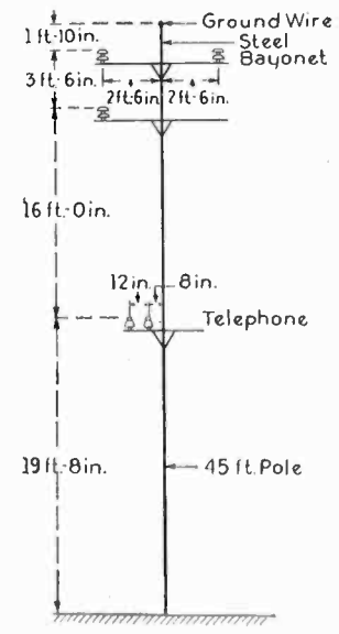
FIG. 10 (B)—ARRANGEMENT OF CONDUCTORS ON THE VIDA-MONTGOMERY SECTION.
