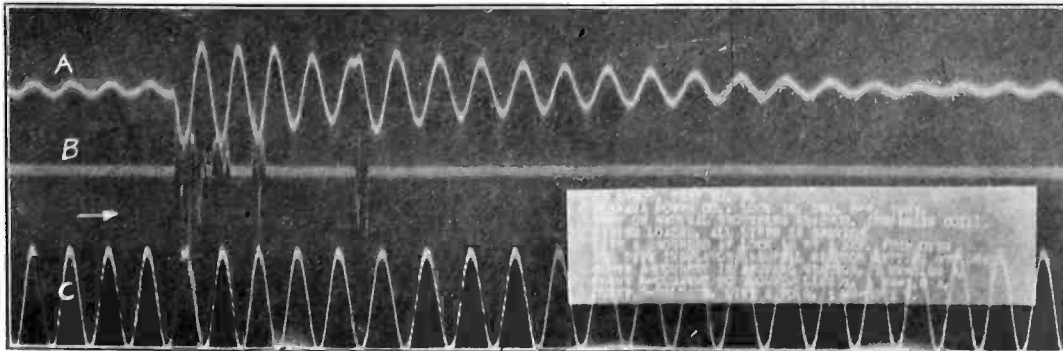
FIG. 31—C D 57307, SYSTEM LOADED, ALL LINES IN SERVICE. CONDUCTOR 1 GROUNDED AT LOCK 12 BY 1 AMPERE FUSE OVER PIN TYPE INSULATOR. NEUTRAL REACTOR SETTING 870 OHMS
