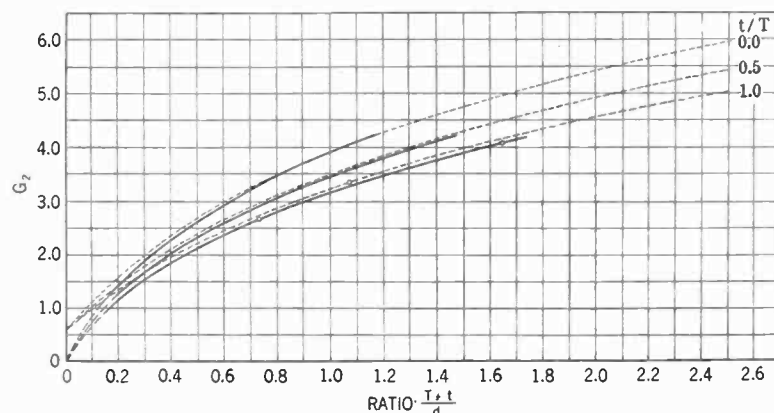
FIG. 4—THE GEOMETRIC FACTOR OF THREE-CONDUCTOR CABLES, UNDER 3-PHASE VOLTAGE
