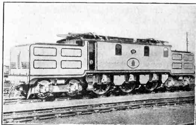
North Eastern Railway, England. Locomotive with geared quill drive. Designed by North Eastern Railway for high-speed service of 75 miles or more per hour. Built by Metropolitan Vickers Co. and North Eastern Railway.
