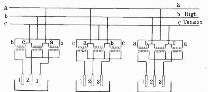
FIG. 9—DISTRIBUTION OF FURNACES TO KEEP HIGH TENSION BALANCED
