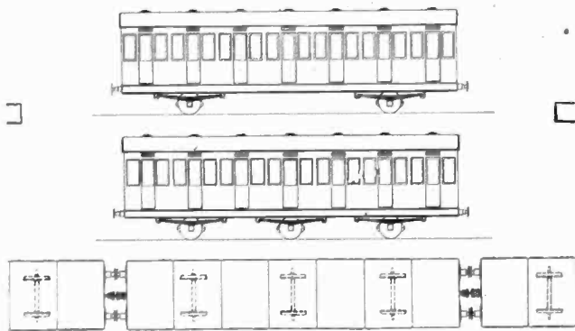
Side elevations of the large two and three-axle cars on European railways. Weight from 20 to 23 tons, seating from 35 to 72 passengers, depending on the class. Over all wheel base 28 to 30 ft. Plan shows arrangement of screw coupler and car buffers.
