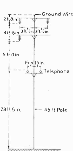
FIG. 10 (A)—ARRANGEMENT OF CONDUCTORS ON LOCK-12-VIDA SELMA SECTION.
