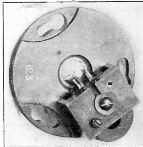
FIG. 3—PHOTOGRAPH OF DIAPHRAGM AND VIBRATING SYSTEM FOR PALLOPHOTOPHONE
