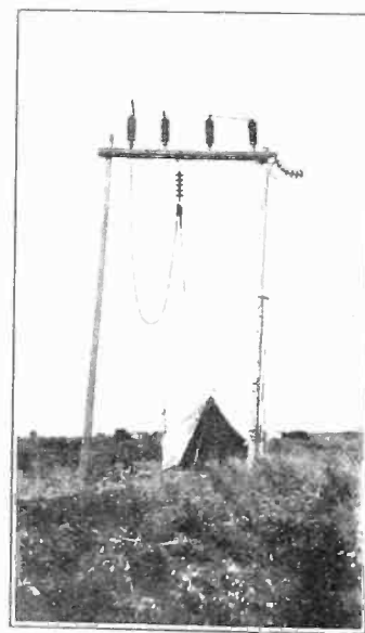
FIG. 4—HIGH-VOLTAGE POTENTIOMETER USED WITH CREST METER
