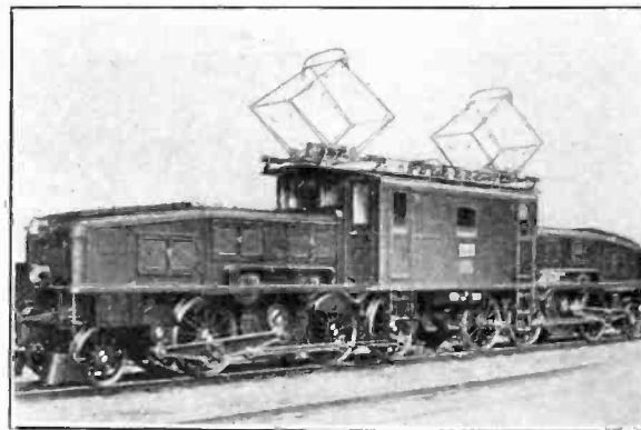
Swiss Federal Railways. Locomotive with geared side rod drive; each of the jack cranks is driven by two motors, the connecting yoke which is attached to the driver, being carried by an idle crank at its outer end. Built by the Oerlikon Co. and the Swiss Locomotive and Machine Works, Winterthur.
