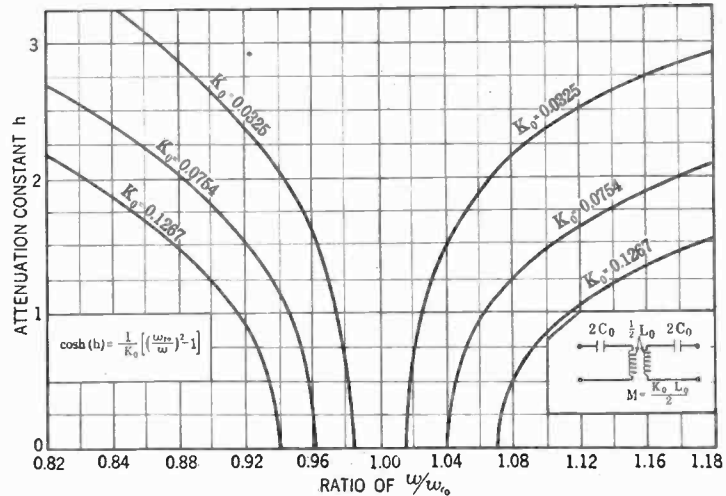
FIG. 8—ATTENUATION CONSTANT CURVES FOR IDEAL FILTER
