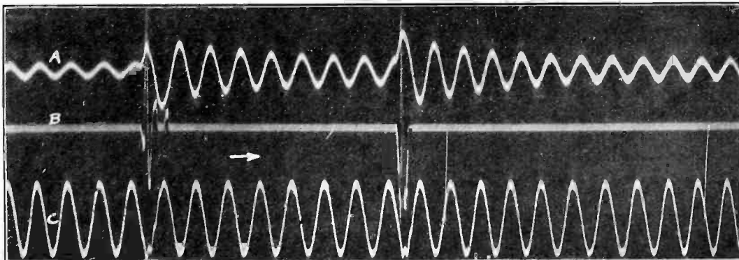
FIG. 30—C D 57306, SYSTEM LOADED, ALL LINES IN SERVICE. CONDUCTOR 1 GROUNDED AT LOCK 12 BY 1 AMPERE FUSE OVER PIN TYPE INSULATOR. NEUTRAL REACTOR SETTING 929 OHMS
