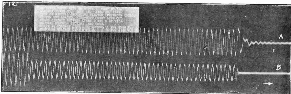
FIG. 47—C D 57372. SYSTEM NOT LOADED. VIDA-MONTGOMERY LINE OUT. NEUTRAL GROUNDED THROUGH REACTOR SET AT 1410 OHMS. SHORT CIRCUIT BETWEEN CONDUCTORS 2 AND 3 AT VIDA Curve A, Voltage from Conductor 1 to ground. Curve B, Voltage between Conductors 2 and 3.
