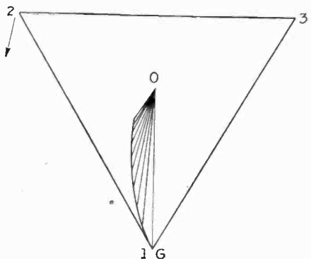
FIG. 41—POLAR DIAGRAM OF VOLTAGE OSCILLATION AFTER BREAKING OF ARC. FROM CD 57305 (FIG. 29). REACTOR SETTING 982 OHMS. FREQUENCY DECREASES FROM 60 TO 59.4 AT INSTANT FUSE BLOWS
