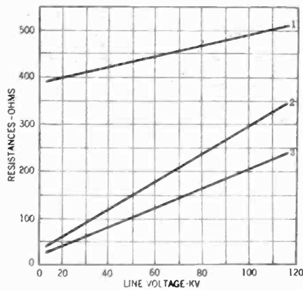
FIG. 3—SURGE IMPEDANCE AND ARRESTER RESISTANCES
