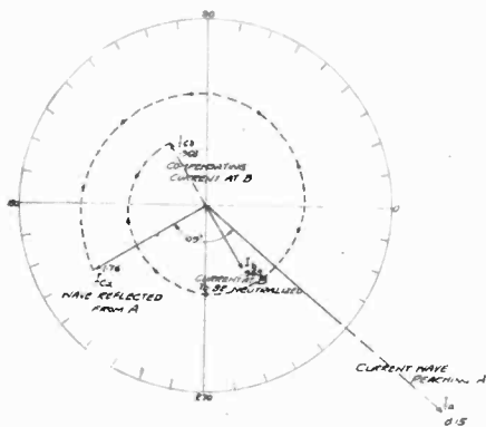
FIG. 43—VECTOR RELATIONS IN COMPENSATION PROBLEM
