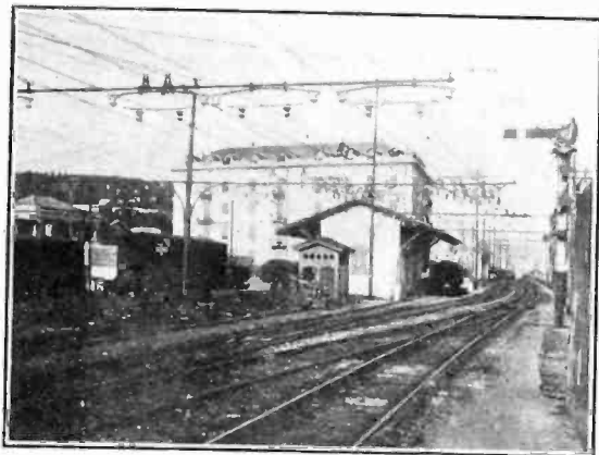
Italian State Railways. View of overhead lines of three-phase system, showing long bracket arm construction and bow shaped supports to facilitate the alinement of the conductors.
