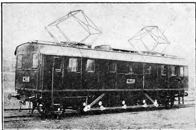
Midi Railway, France. Locomotive with direct-connected side rod drive with two motors connected to jack cranks, exterior to the driving wheels. Built by C. F. T. H., Paris, and the Swiss Locomotive and Machine Works, Winterthur.
