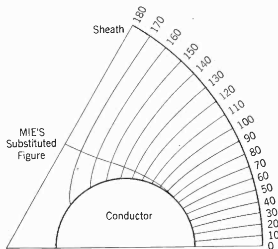
FIG. 3—FIGURE FOR GRAPHICAL CORRECTION OF THREE-CONDUCTOR CABLE
