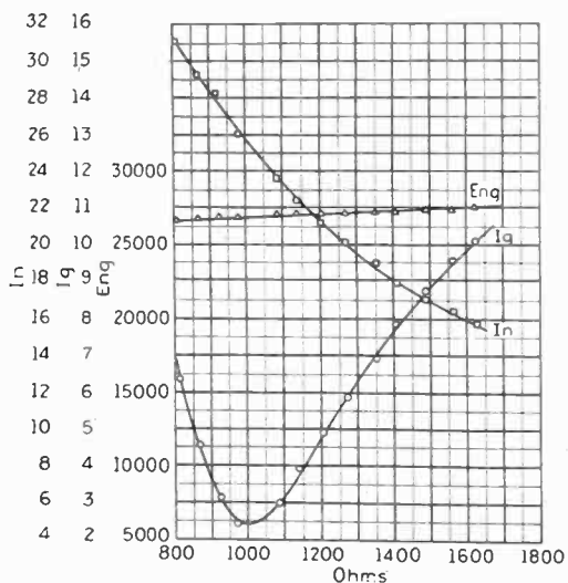
FIG. 23—RESONANCE CURVE, SYSTEM LOADED, ALL CIRCUITS IN. CONDUCTOR 1 GROUNDED AT LOCK 12. DRY WEATHER CONDITIONS
