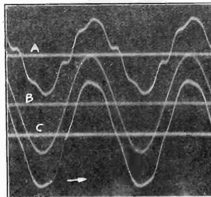
FIG. 20—C D 57293, TEST 7, LINE CHARGED, NO LOAD, REACTOR BETWEEN NEUTRAL AND GROUND. CONDUCTOR 1 SOLIDLY GROUNDED AT SELMA
