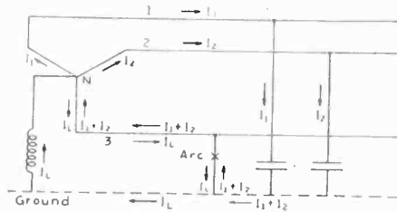
FIG. 3—THREE-PHASE SYSTEM WITH REACTOR BETWEEN NEUTRAL AND GROUND. FIGURE SHOWS FLOW OF CURRENTS WITH ARC FROM PHASE 3 TO GROUND
