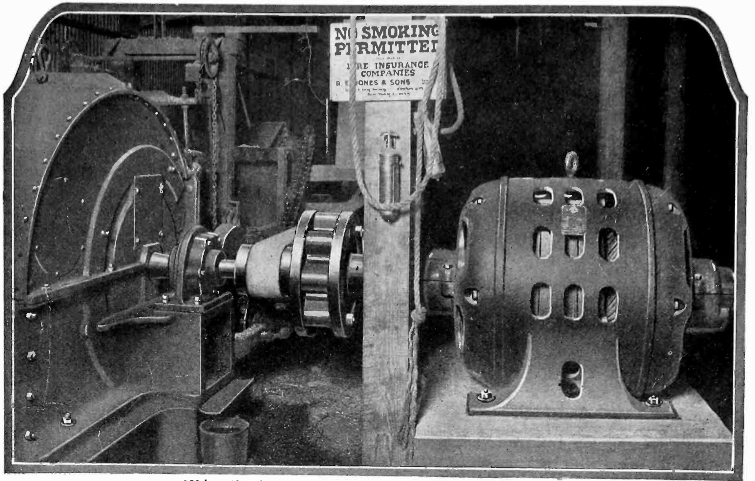
150 hp.—60 cycle—440 volt Type BR. Wagner Motor operating alfalfa chopper
