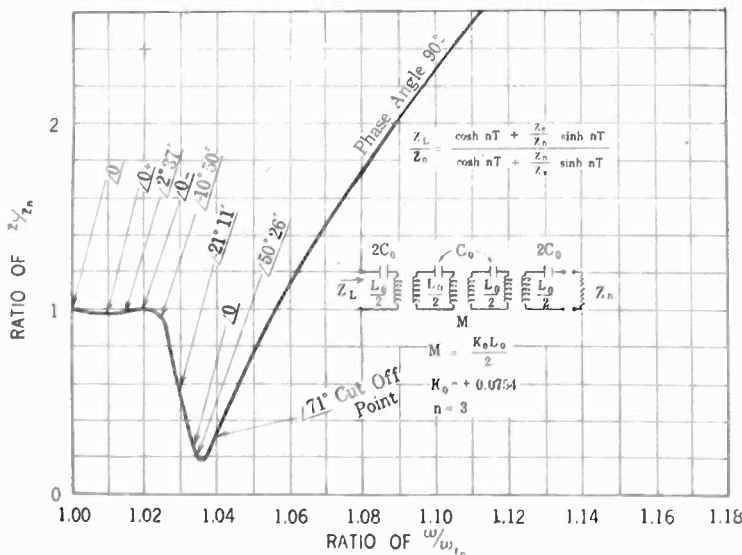
FIG. 10—IDEAL FILTER LINE IMPEDANCE
