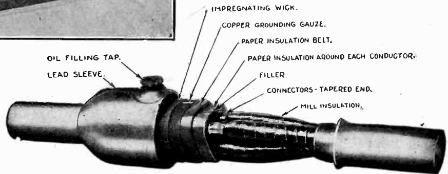
Detailed View Metropolitan Oil-Filled Cable Joint
