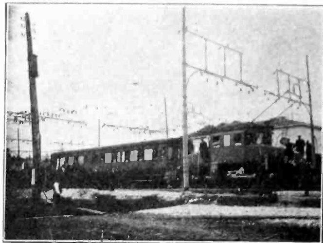
Italian State Railways. Locomotive with direct connected side rod drive with two motors connected to a Scotch yoke. Originally built by the Italian Westinghouse Vado Ligure Works. A large number of locomotives with similar drive has since been built by other Italian manufacturers.
