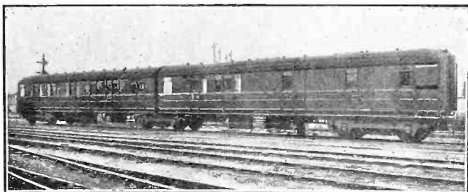
Great Northern Railway, England. Two articulated cars showing the intermediate truck midway between the cars. Groups of five cars, similarly articulated, are in regular main line service.
