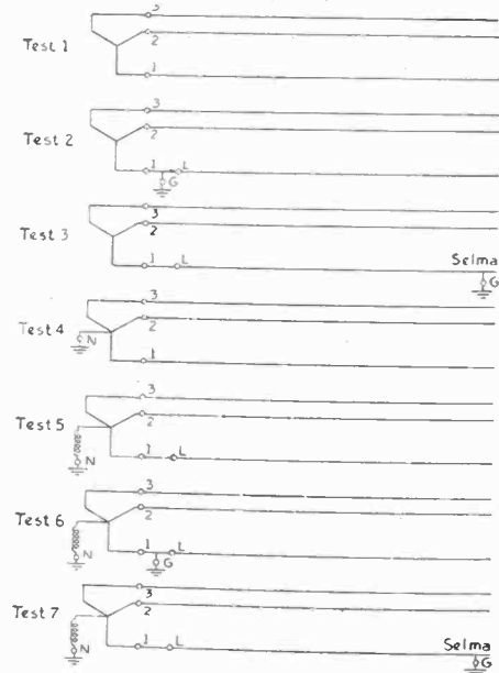
FIG. 16—DIAGRAM OF CONNECTIONS FOR TESTS 1 TO 7 INCLUSIVE MADE UNDER STEADY CONDITIONS
