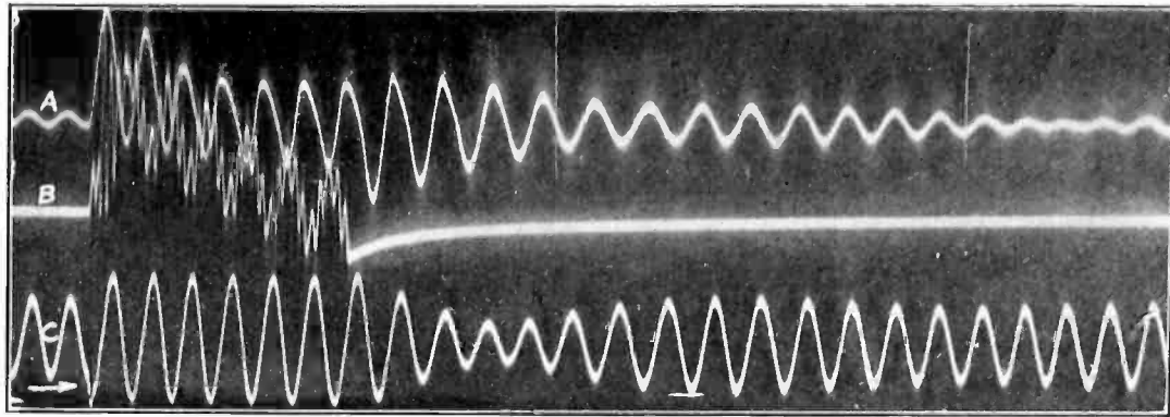
FIG. 45—C D 57368. SYSTEM LOADED. ALL LINES IN SERVICE. CONDUCTOR 1 GROUNDED AT LOCK 12 BY 1 AMPERE FUSE ACROSS 3.5 INCH HORN GAP. NEUTRAL REACTOR SETTING 1207 OHMS Curve A, Current in Neutral Reactor. Curve B, Current from Conductor 1 to ground. Curve C, Voltage from Conductor 3 to ground.
