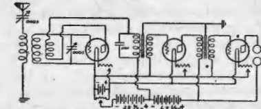
Standard vacuum tube detector and two-stage audio-frequency amplifier (vacuum using heavy wire with No. 75 for primary, No. 50 for secondary and No. 25 for resistor; potentiometer across "B" battery 400 ohms; audio-amplifying transformers 5 to 1 ratio)
