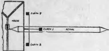
Fig. 3. An arrangement of three earth connections which gives good results.
