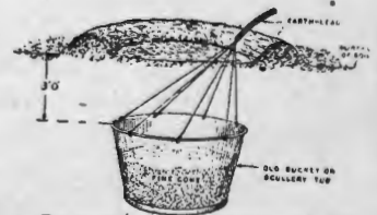
Fig. 2. A very good type of earth connection.
