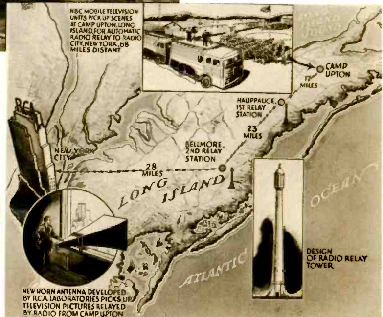
Automatic radio-relay stations developed by RCA are used to "bounce" television programs and other communications on ultra-short waves from city to city.
