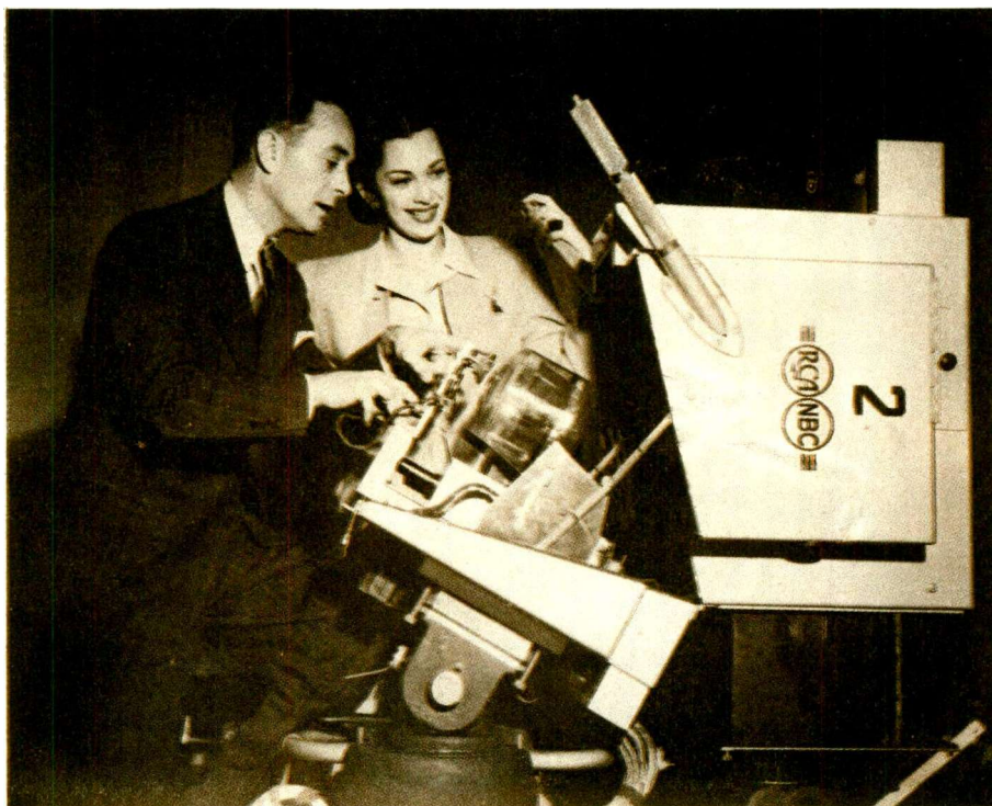
The television camera uses the Iconoscope as its “eye,” perfected in RCA Laboratories.
