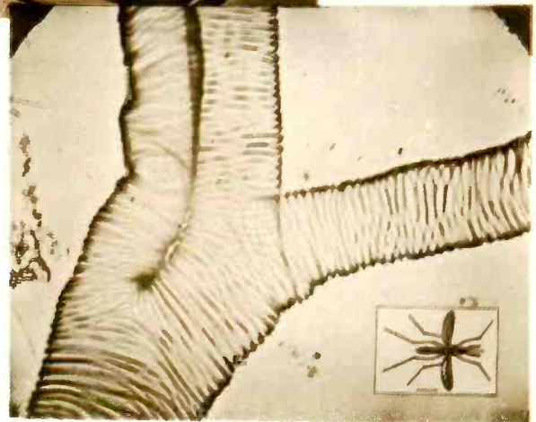
Console model of the RCA electron microscope enables photographic enlargement up to 100,000 diameters, depending on the subject matter. RIGHT: The windpipe of a mosquito magnified 65,000 times.
