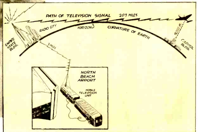
A radio-equipped airplane looked-in on New York by television from an altitude of 18,000 feet over the Capitol in Washington. Diagram illustrates the performance of the ultra-short waves.
