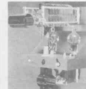
LEFT: W6ITH, top voice man, has a power amplifier that is a symbol of symmetry. Note that corresponding plate and grid leads are identical in length and as short as is mechanically possible. RIGHT: W2IOP's layout, using a single 814, pulled in the biggest score for a single operator in history. 93% of W2IOP's 40 tubes are RCA!
