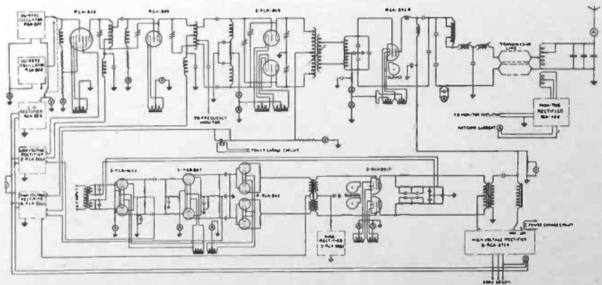
Simplified Schematic Diagram of the 5-DX Transmitter.
