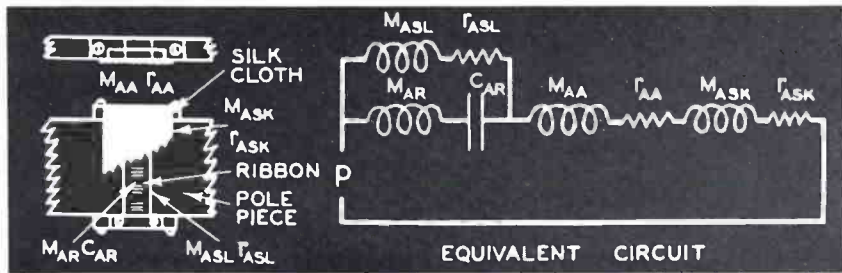
Fig. 9. The elements of the velocity microphone and the equivalent electrical circuit of the acoustical system. M_{AR} inertance of the ribbon. C_{AR} acoustic capacitance of the ribbon. M_{ASL} inertance of the slit between the ribbon and pole pieces. r_{ASL} acoustic resistance of the slit between the ribbon and pole pieces. M_{AA} inertance of the air load upon the ribbon. r_{AA} acoustic resistance of the air load upon the ribbon. M_{ASK} inertance of the silk covering the ribbon. r_{ASK} acoustic resistance of the silk covering the ribbon. p driving sound pressure.
