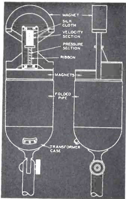
Fig. 1. Uni-directional microphone with the screen removed.
