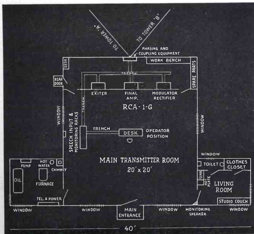
Floor plan of WHBF transmitter station.
