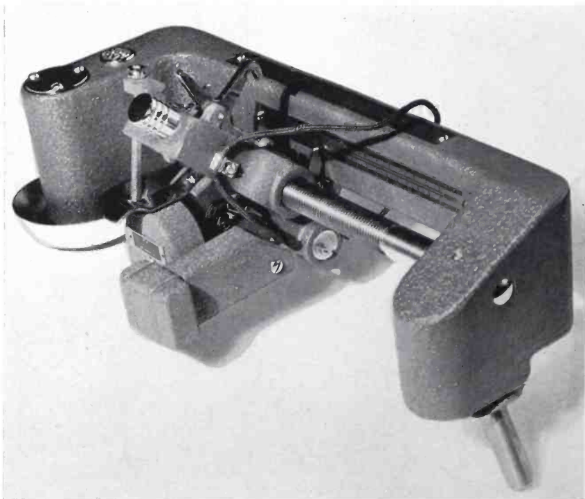
Fig. 4. The RCA 72-B Recording Attachment equipped with MI-4881A cutter head is available for use with the 70-B turntable.
